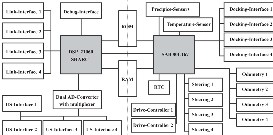
Fig. 4. Schematic overview over the CALINCA-vehicle electronics
