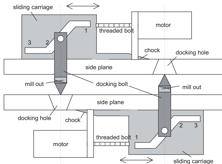
Fig. 3: Mechanical docking mechanism
