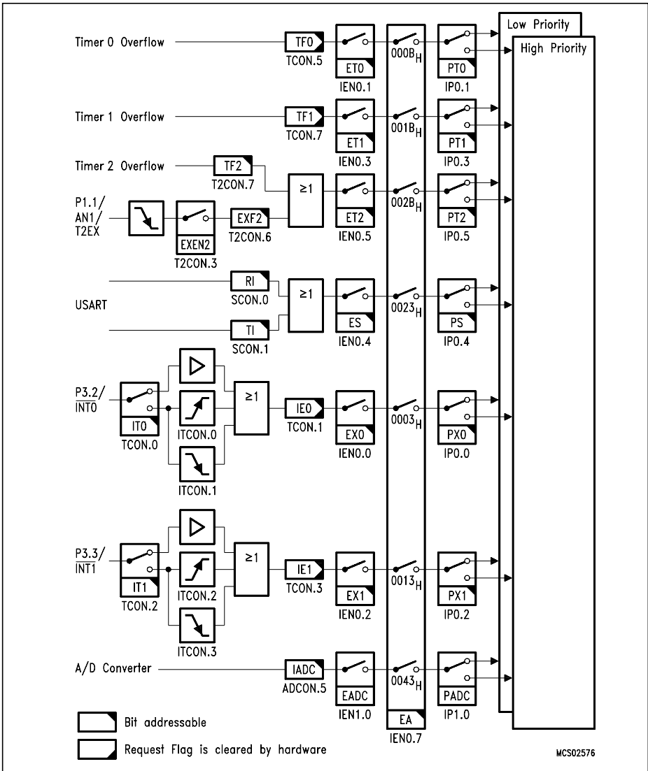
Figure 11 Interrupt Request Sources (Part 1)
