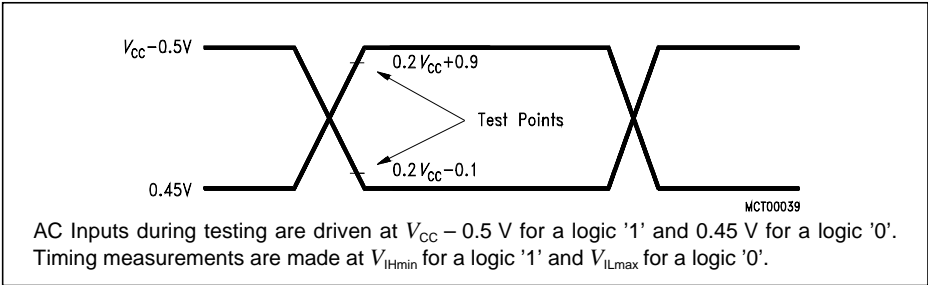
Figure 21 AC Testing: Input, Output Waveforms
