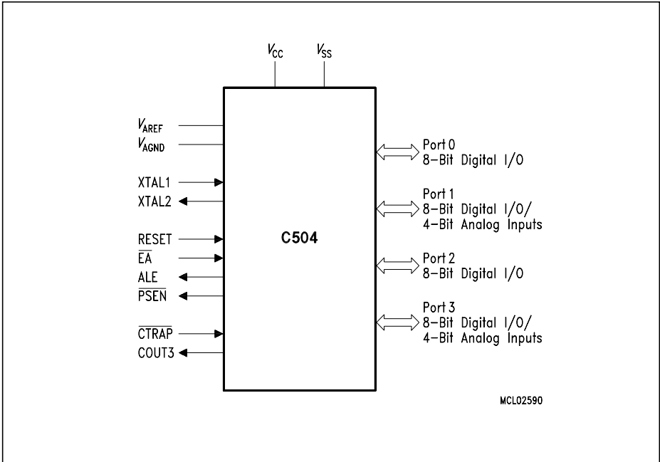
Figure 1 Logic Symbol
