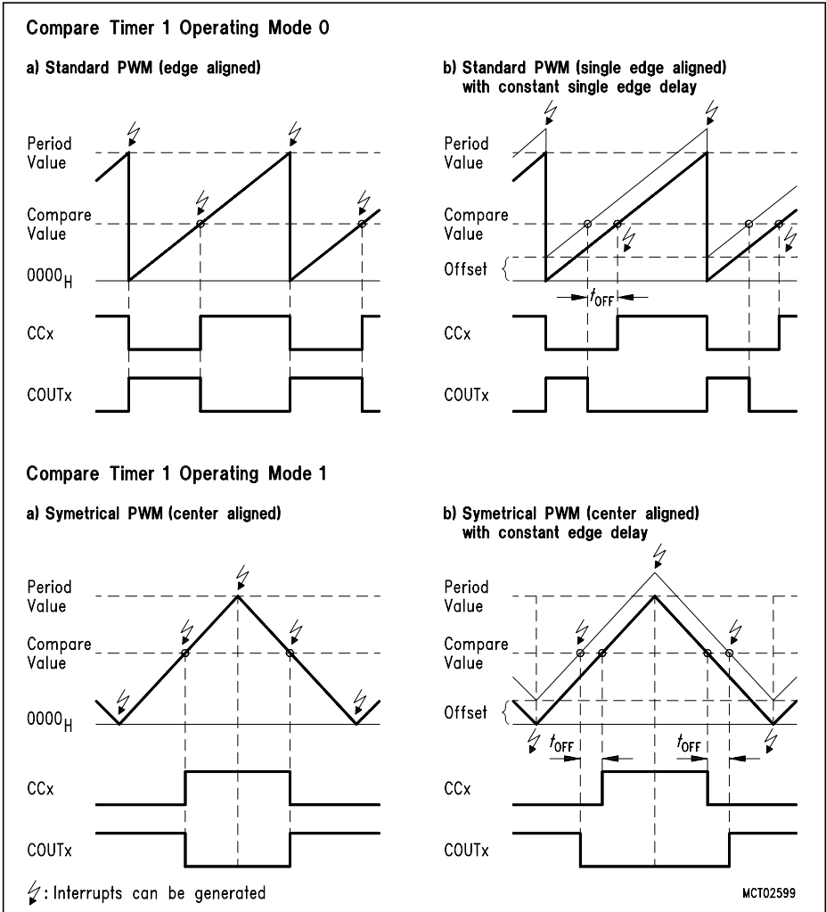
Figure 7 Basic Operating Modes of the CAPCOM Unit
