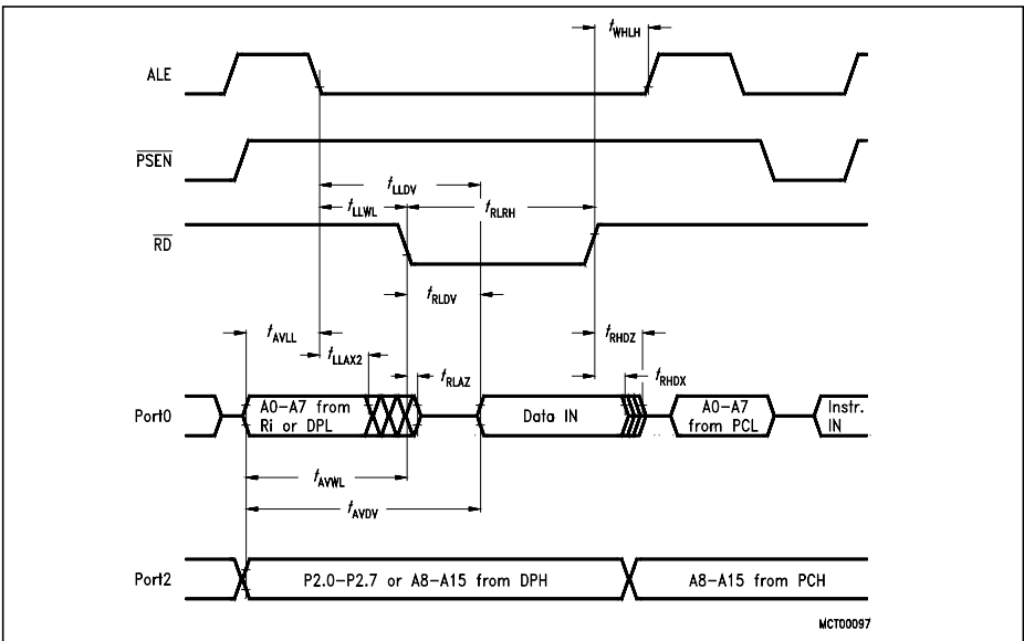
Figure 16 Data Memory Read Cycle
