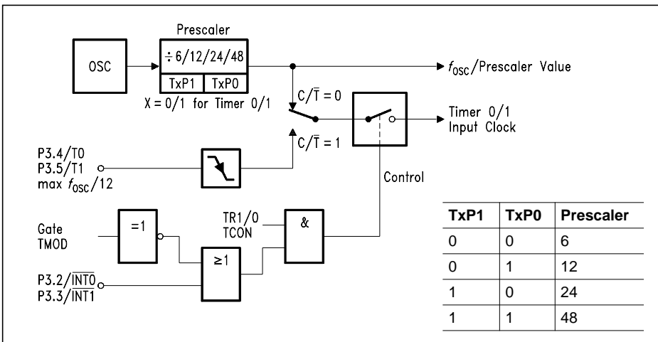
Figure 17 Timer/Counter 0 and 1 Input Clock Logic
