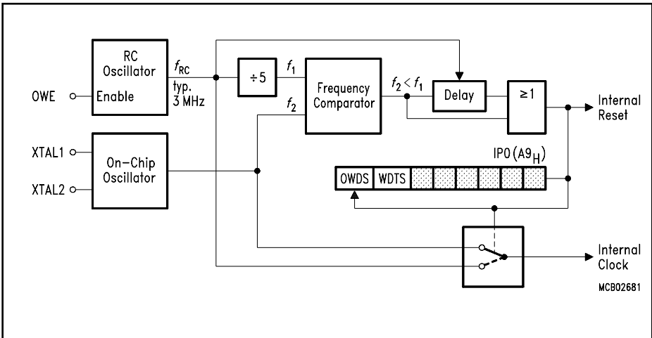
Figure 35 Block Diagram of the Oscillator Watchdog
