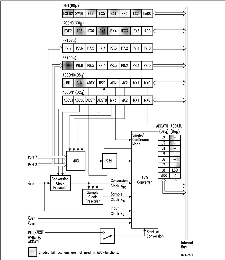
Figure 27 A/D Converter Block Diagram
