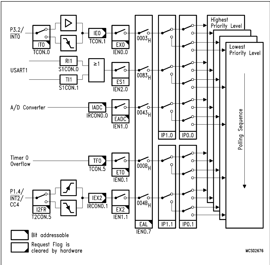
Figure 30 Interrupt Request Sources (Part 1)
