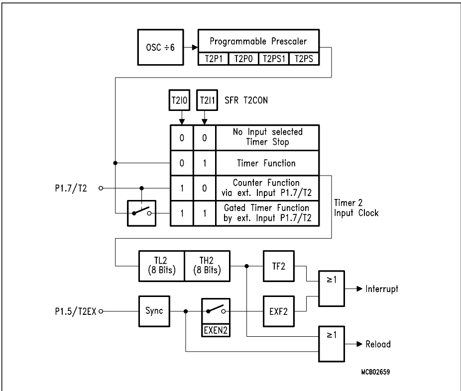
Figure 19 Block Diagram of Timer 2
