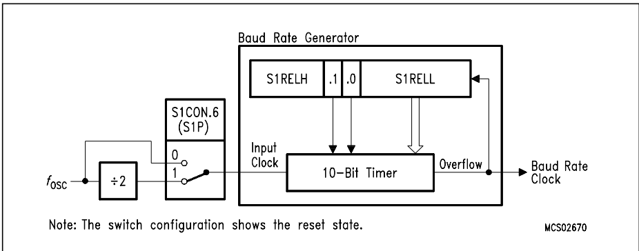
Figure 26 Serial Interface 1 : Baud Rate Generator Configuration
