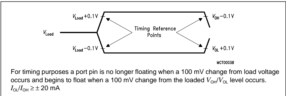
Figure 41 AC Testing: Float Waveforms
