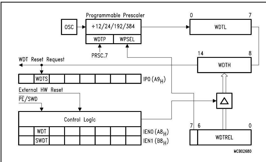
Figure 34 Block Diagram of the Programmable Watchdog Timer
