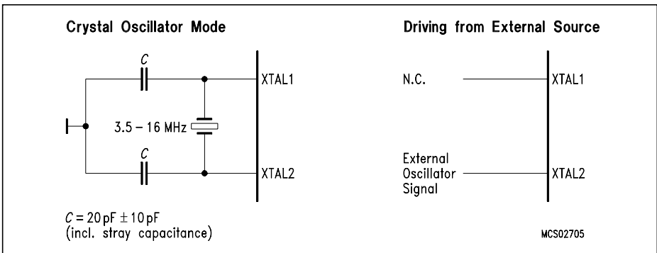
Figure 13 Recommended Oscillator Circuitries
