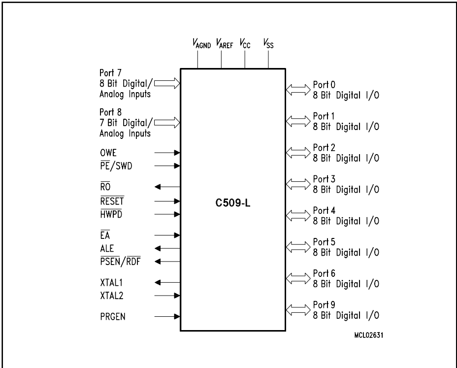
Figure 2 Logic Symbol
