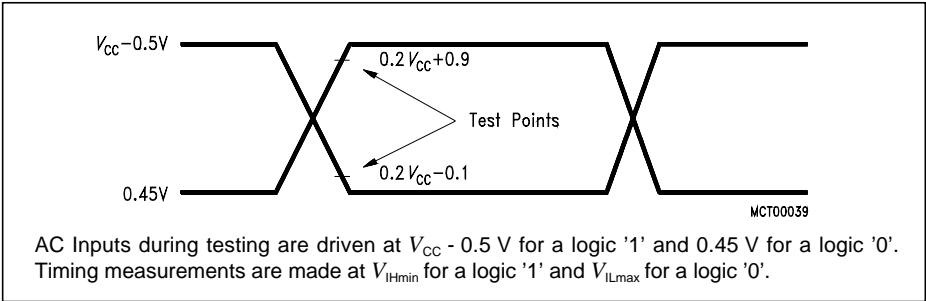
Figure 40 AC Testing: Input, Output Waveforms
