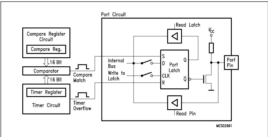
Figure 21 Port Latch in Compare Mode 0
