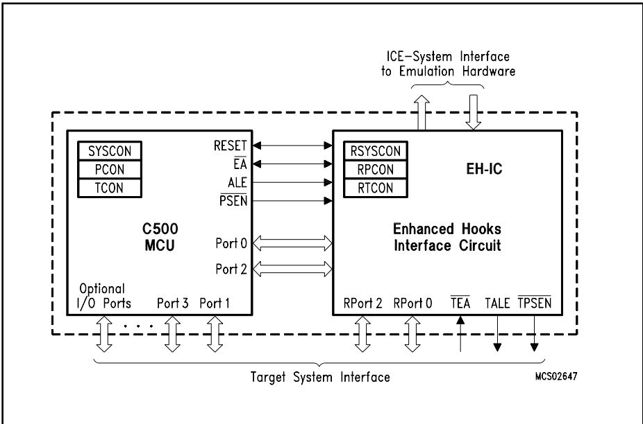
Figure 15 Basic C500 MCU Enhanced Hooks Concept Configuration
