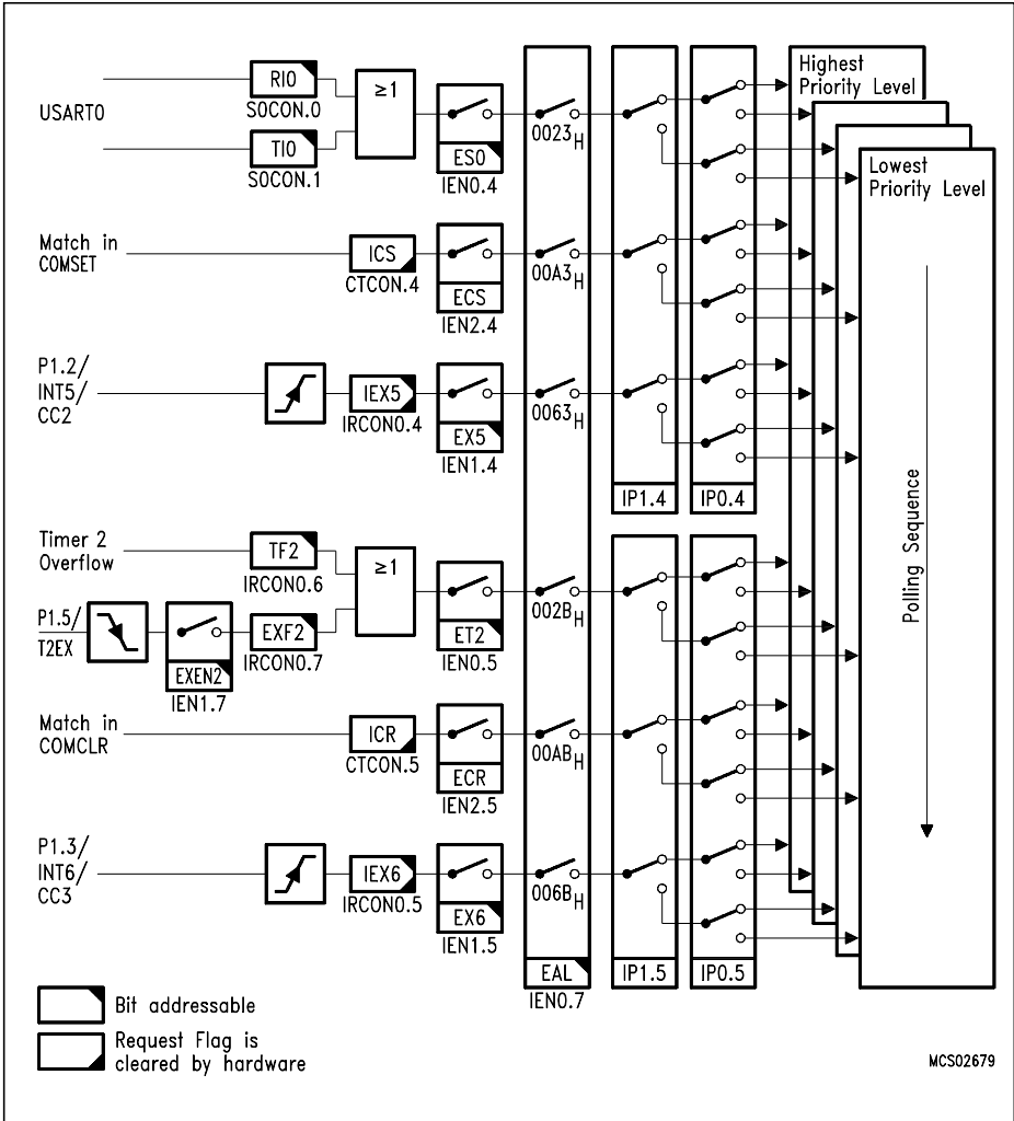
Figure 33 Interrupt Request Sources (Part 4)
