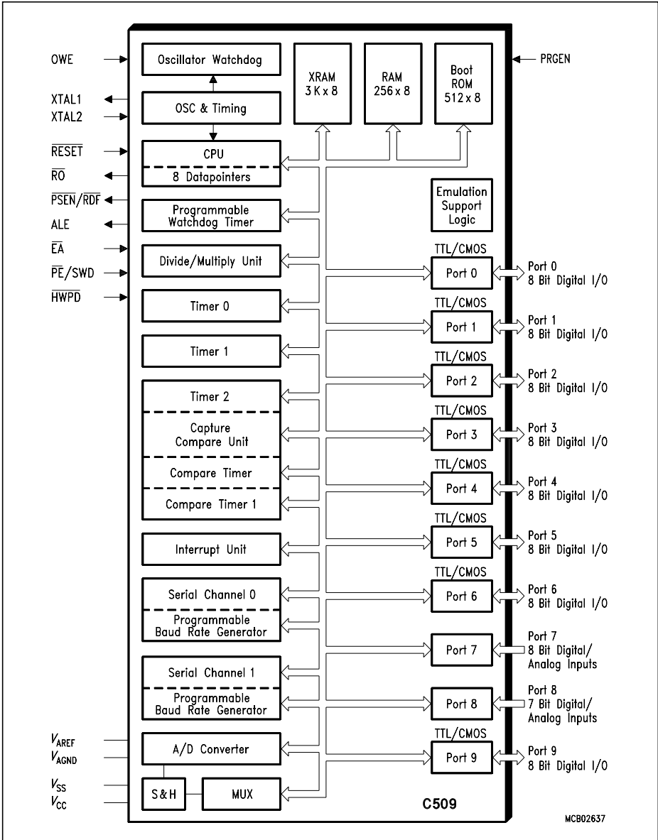
Figure 4 Block Diagram of the C509-L
