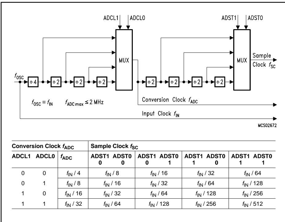
Figure 28 A/D Converter Clock Selection
