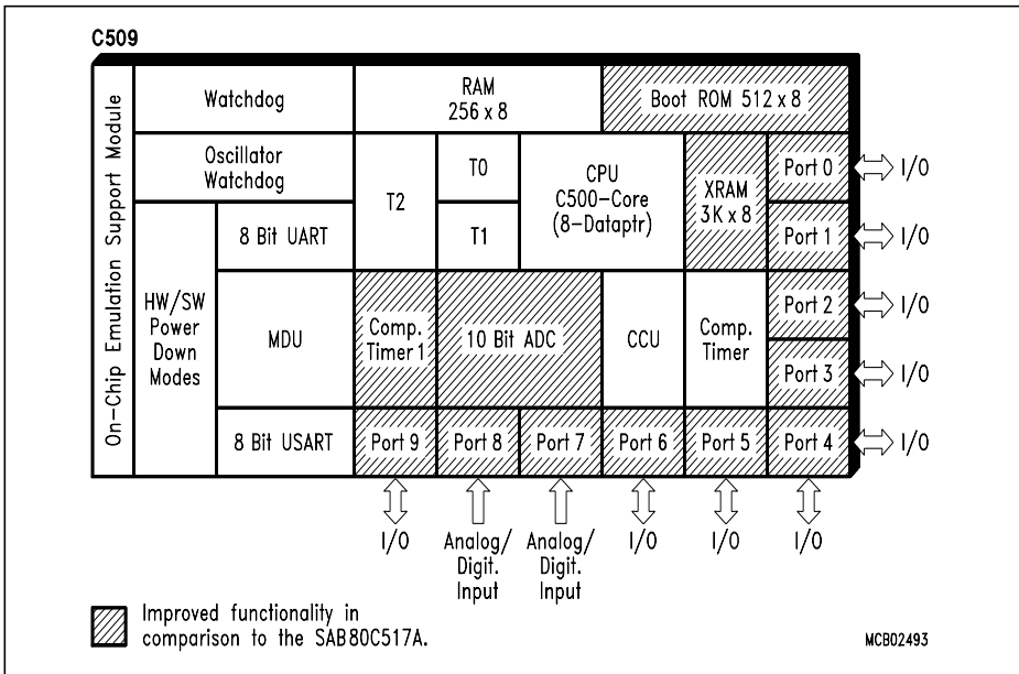
Figure 1 C509-L Functional Units
