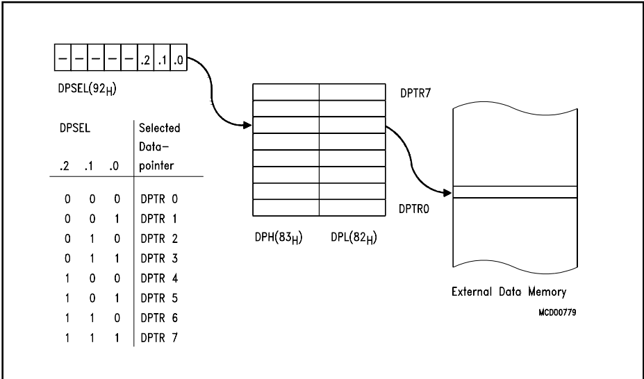
Figure 14 External Data Memory Addressing using Multiple Datapointers
