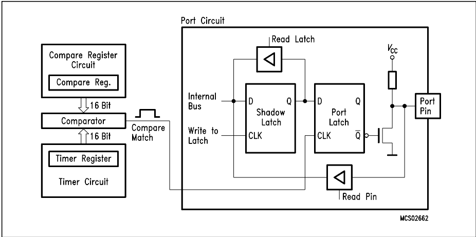
Figure 22 Compare Function in Compare Mode 1
