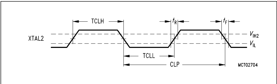
Figure 39 External Clock Drive Drive XTAL2
