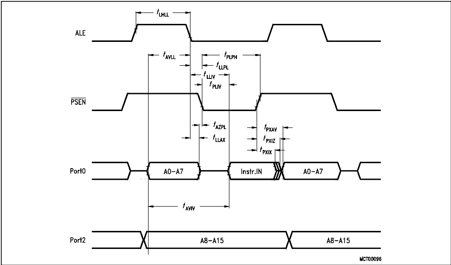
Figure 36 Program Memory Read Cycle
