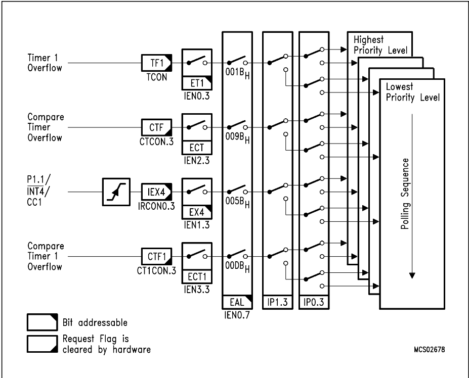
Figure 32 Interrupt Request Sources (Part 3)
