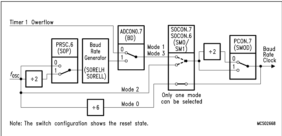
Figure 25 Serial Interface 0 : Baud Rate Generation Configuration
