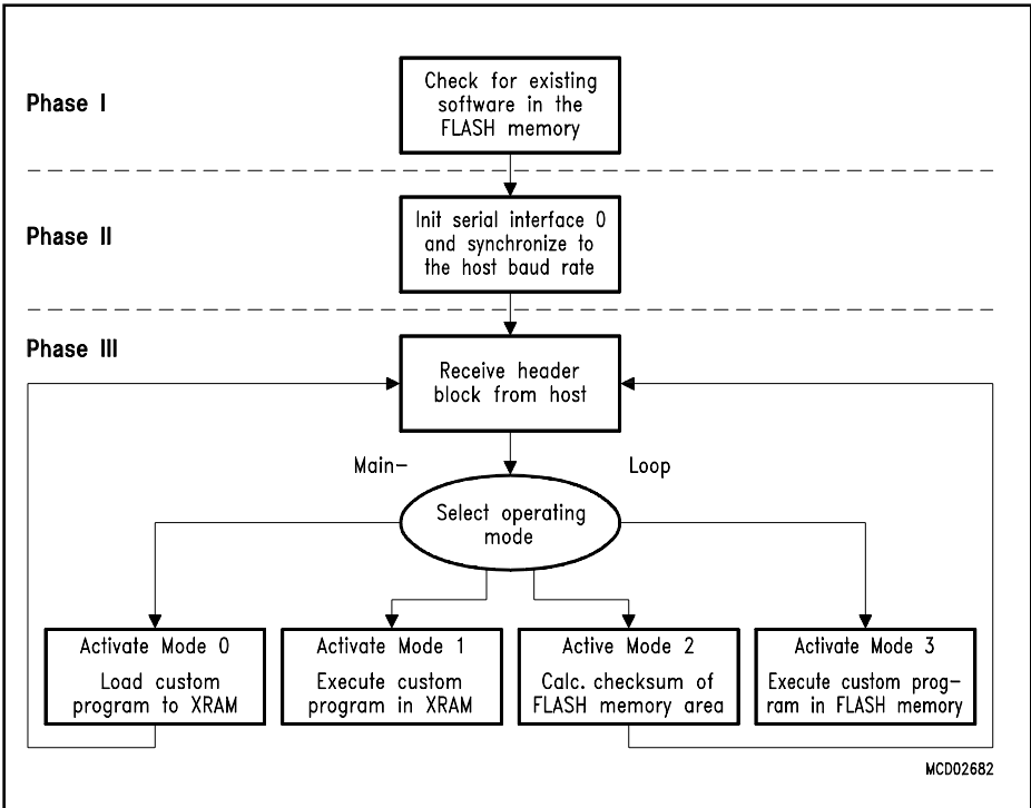
Figure 10 The Three Phases of the Bootstrap Loader
