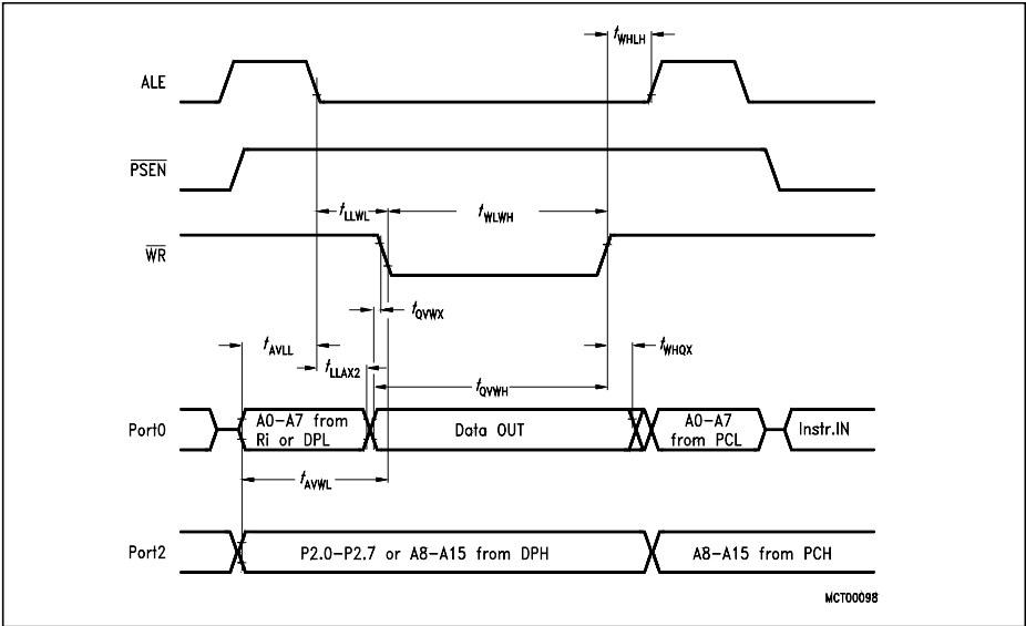
Figure 38 Data Memory Write Cycle
