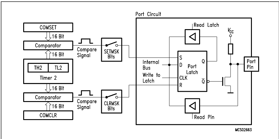
Figure 23 Compare Function of Compare Mode 2
