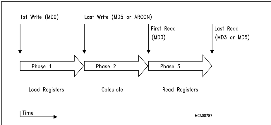
Figure 24 Operating Phases of the MDU
