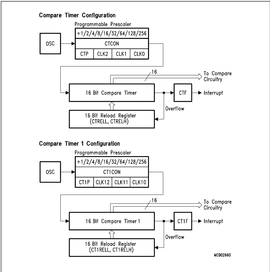
Figure 20 Compare Timer and Compare Timer 1 Block Diagram
