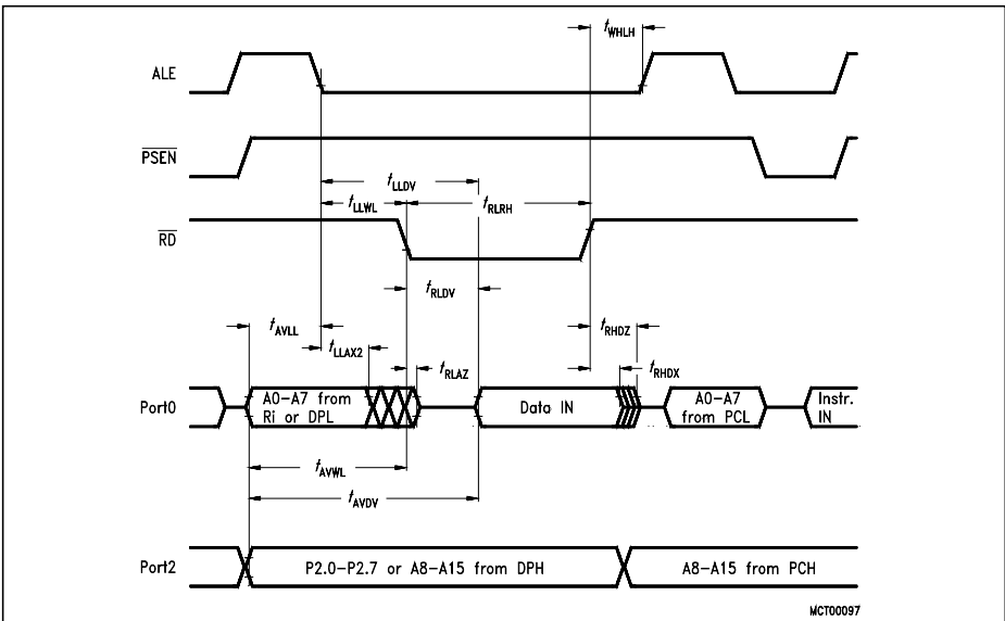
Figure 37 Data Memory Read Cycle
