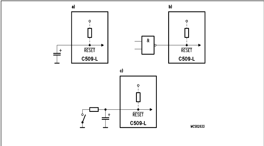
Figure 12 Reset Circuitries
