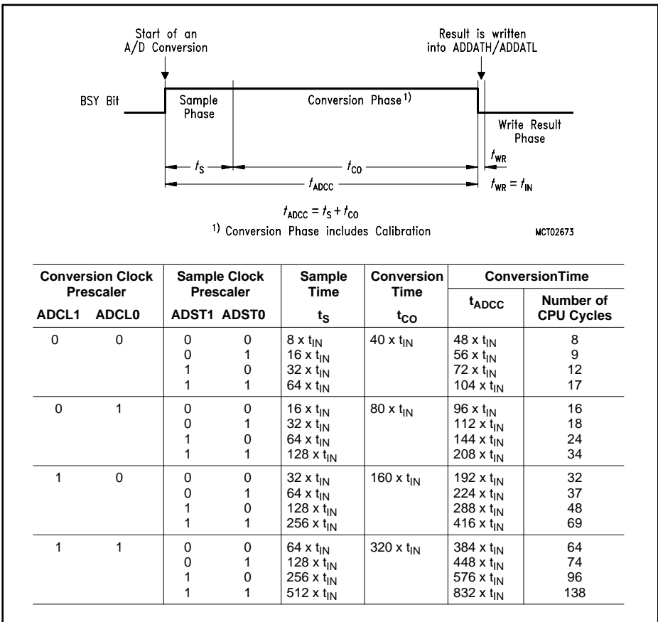
Figure 29 A/D Conversion Timing
