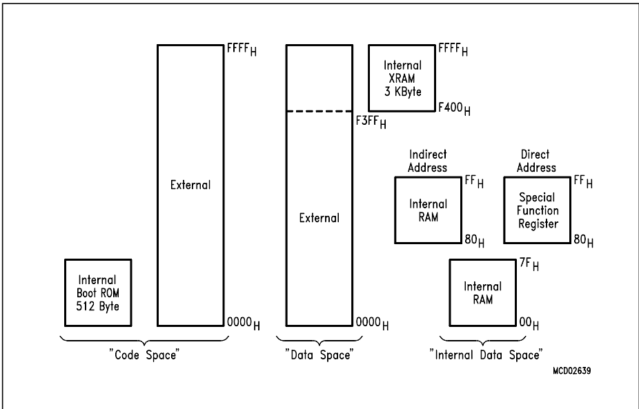
Figure 5 C509-L Memory Map
