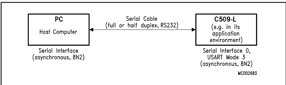
Figure 11 Bootstrap Loader Interface to the PC
