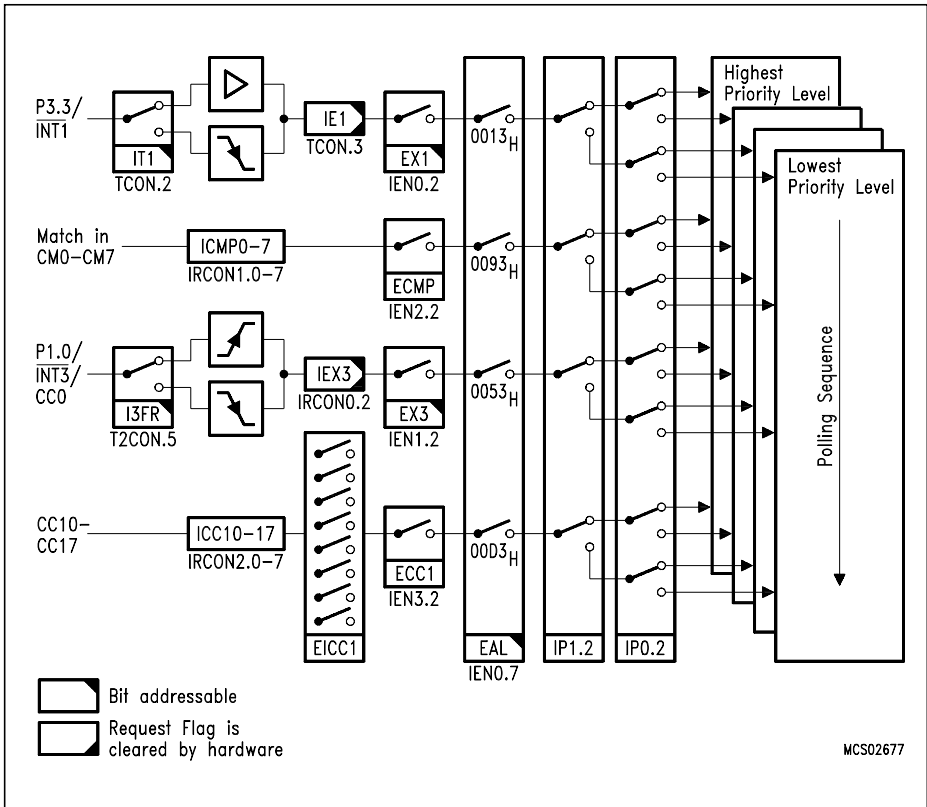
Figure 31 Interrupt Request Sources (Part 2)
