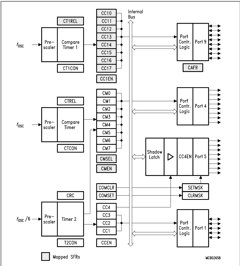
Figure 18 Block Diagram of the CCU
