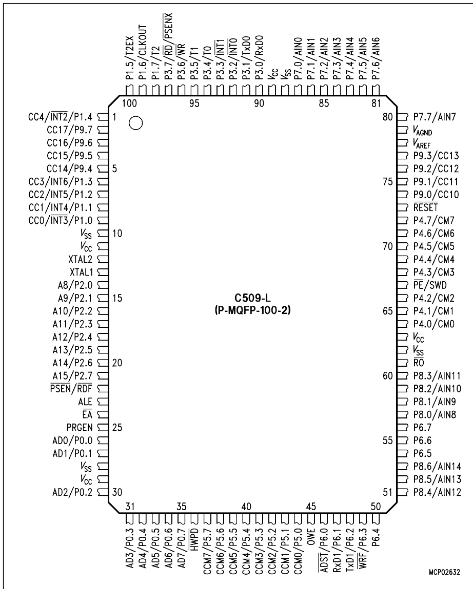
Figure 3 C509-L Pin Configuration (P-MQFP-100-2, Top View)
