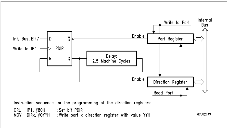
Figure 16 Port Register, Direction Register
