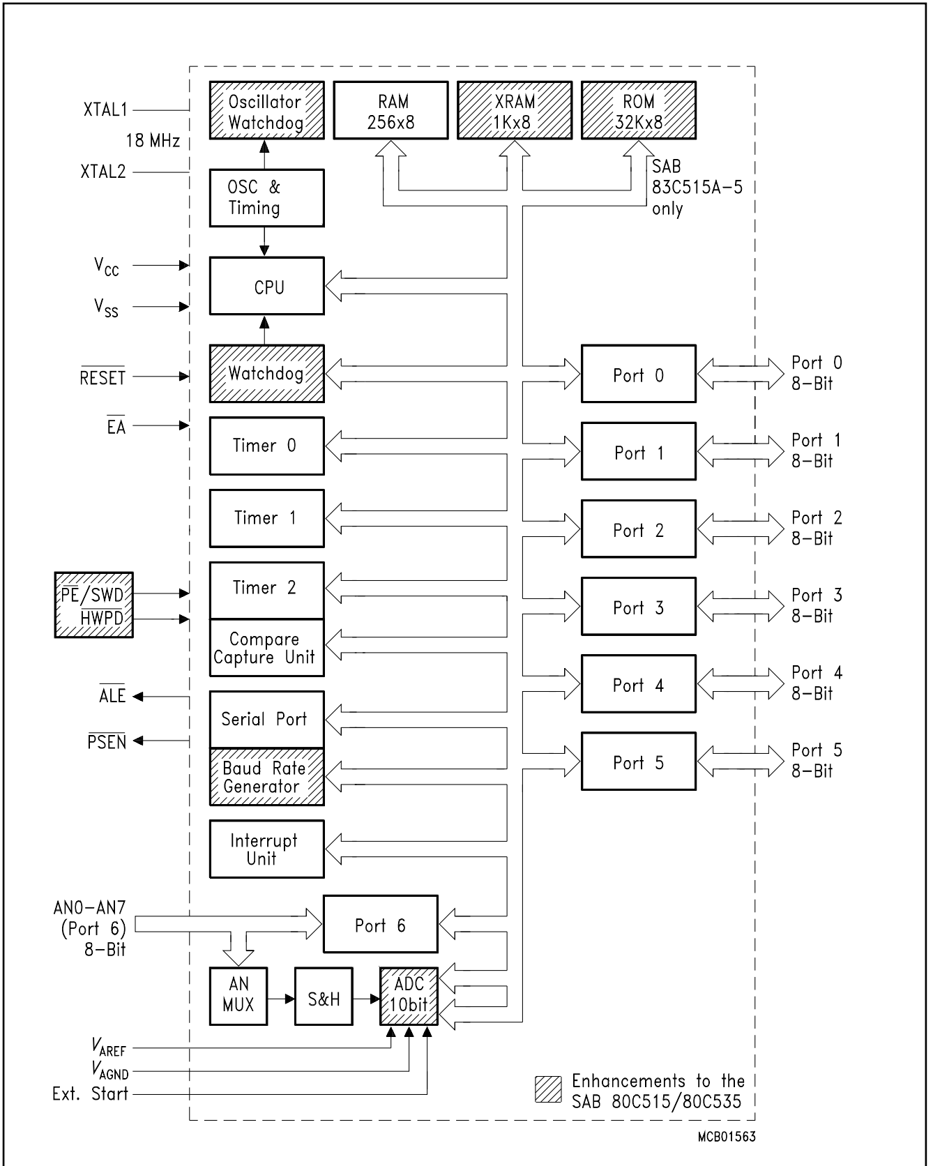
Figure 1 Block Diagram
