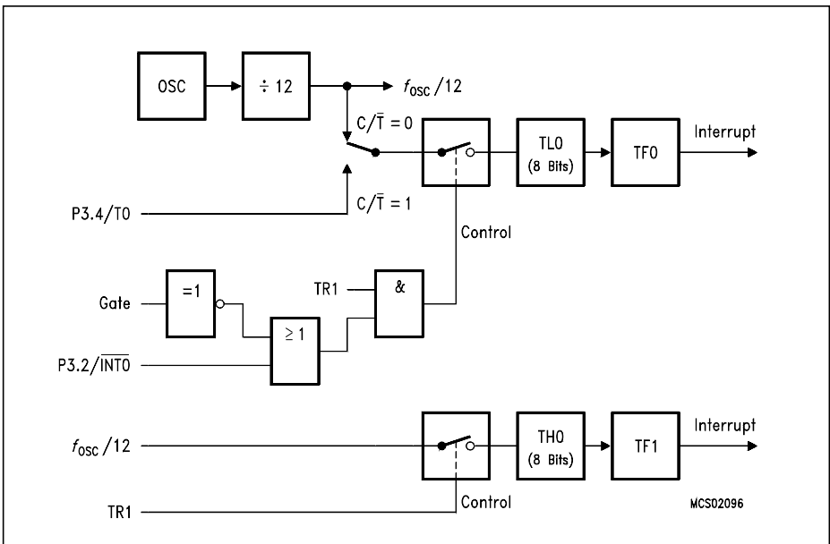
Figure 6-10 Timer/Counter 0, Mode 3: Two 8-Bit Timers/Counters
