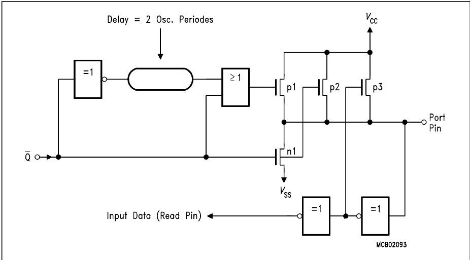
Figure 6-3 Output Driver Circuit of Ports 1, 2 and 3
