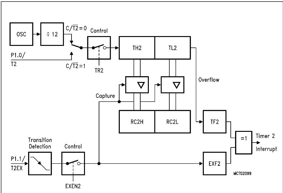
Figure 6-13 Timer 2 in Capture Mode
