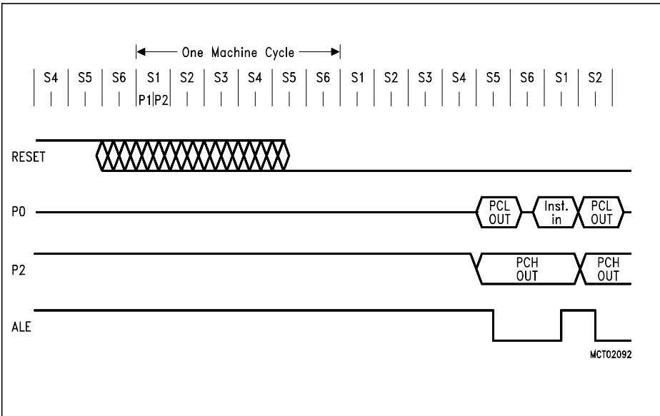
Figure 5-1 CPU Timing after Reset
