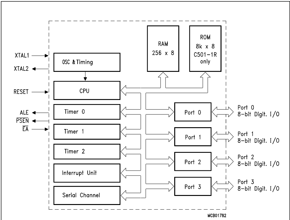
Figure 2-1 Block Diagram of the SAB-C501
