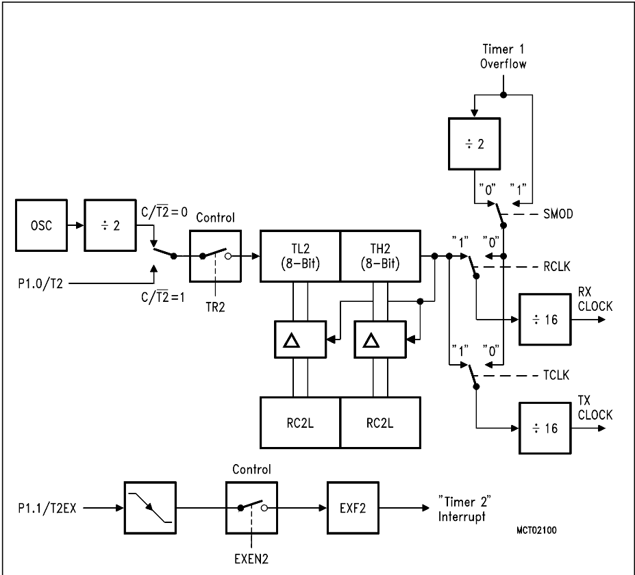
Figure 6-14 Timer 2 in Baud Rate Generator Mode
