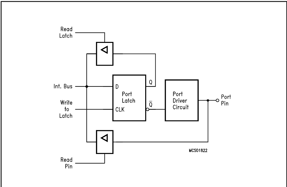
Figure 6-1 Basic Structure of a Port Circuitry
