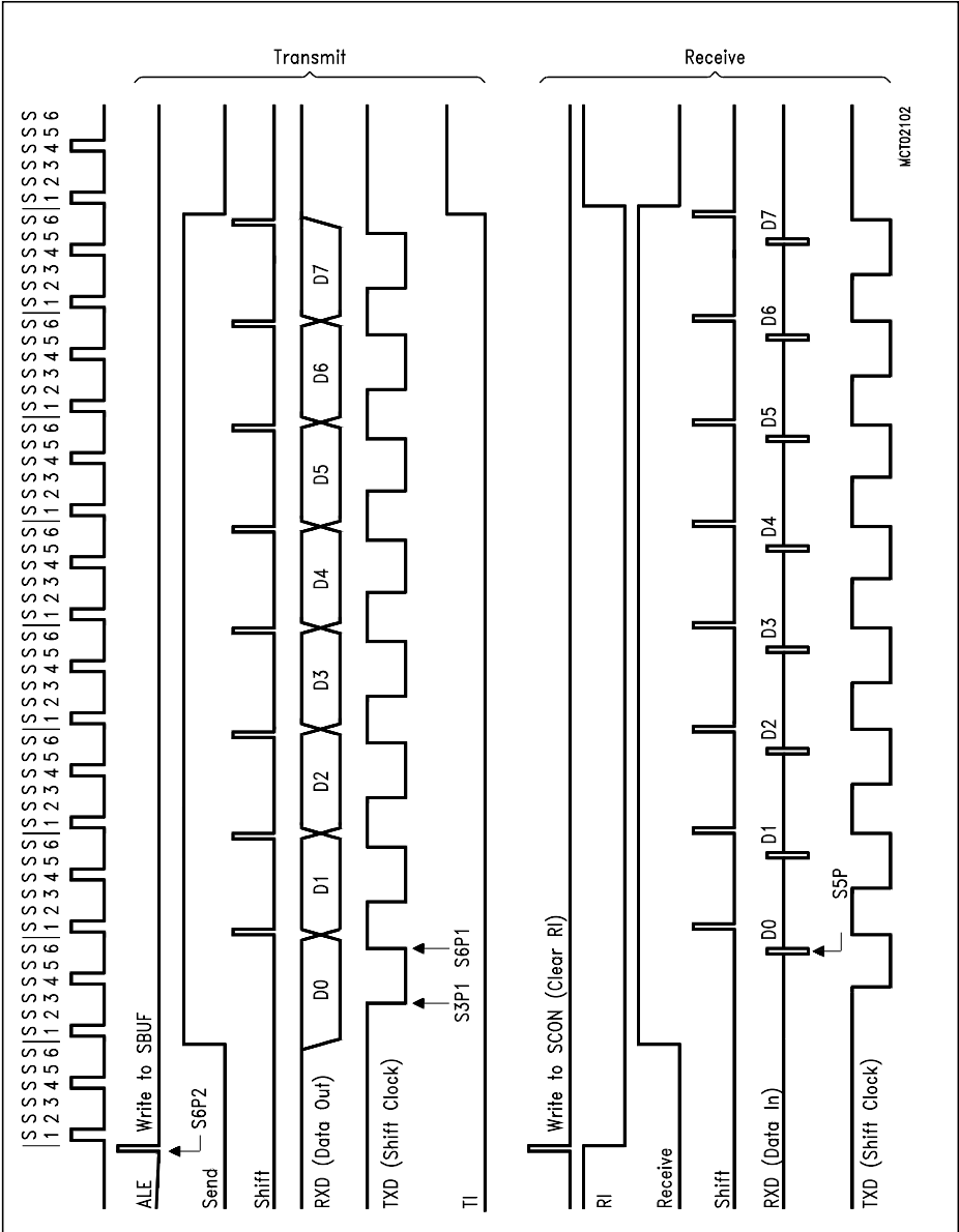
Figure 6-15b Serial Interface, Mode 0, Timing Diagram
