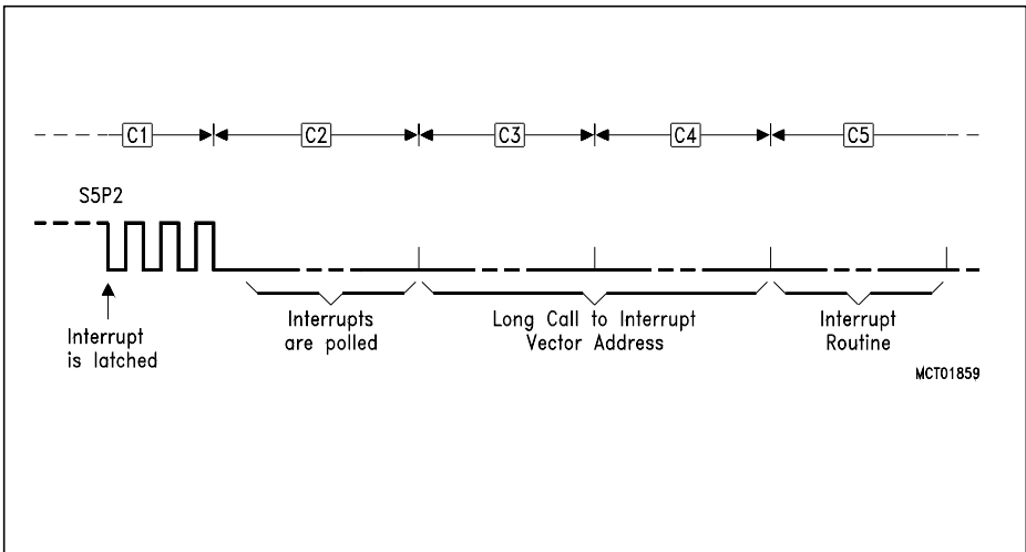
Figure 7-2 Interrupt Response Timing Diagram
