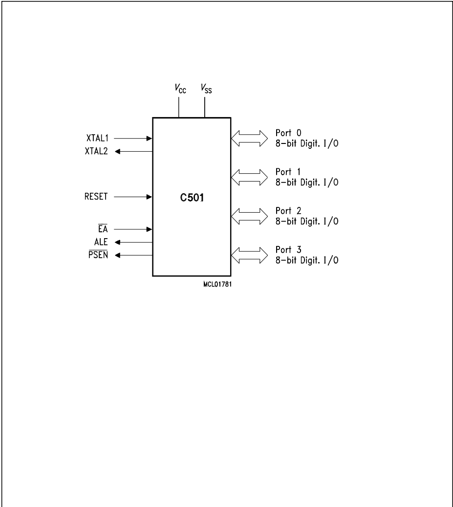
Logic Symbol
