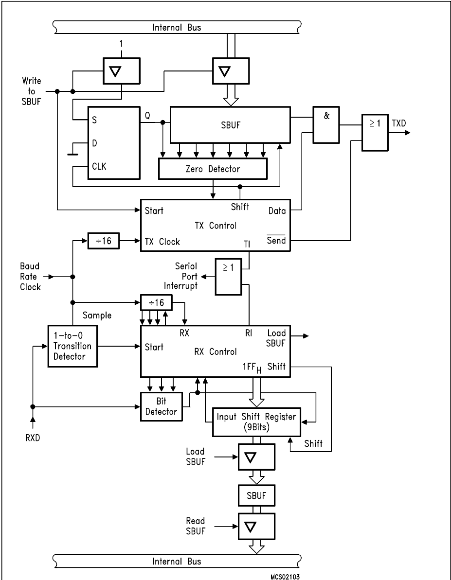
Figure 6-16a Serial Interface, Mode 1, Functional Diagram
