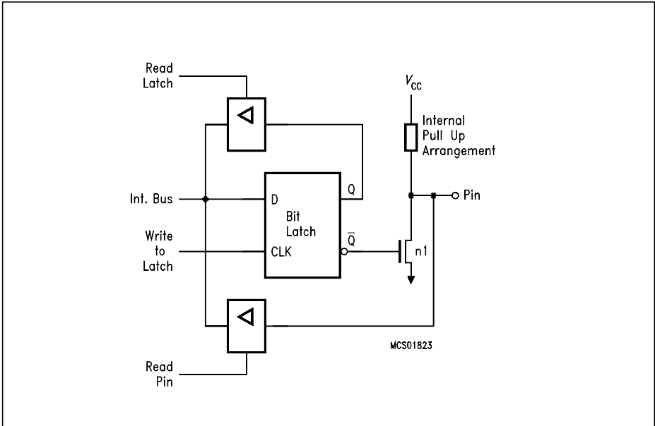
Figure 6-2 Basic Output Driver Circuit of Ports 1, 2 and 3
