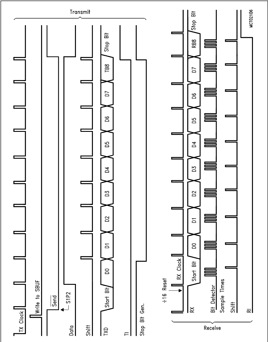
Figure 6-17b Serial Interface, Mode 2 and 3, Timing Diagram
