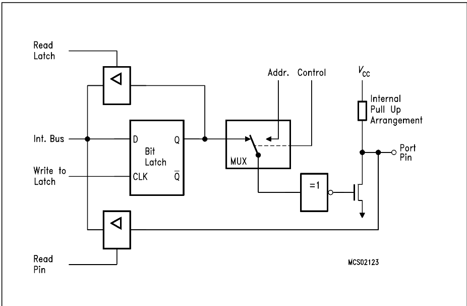
Figure 6-4b Port 2 Circuitry
