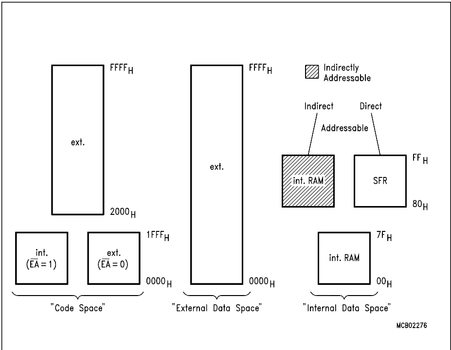
Figure 3-1 Memory Map
