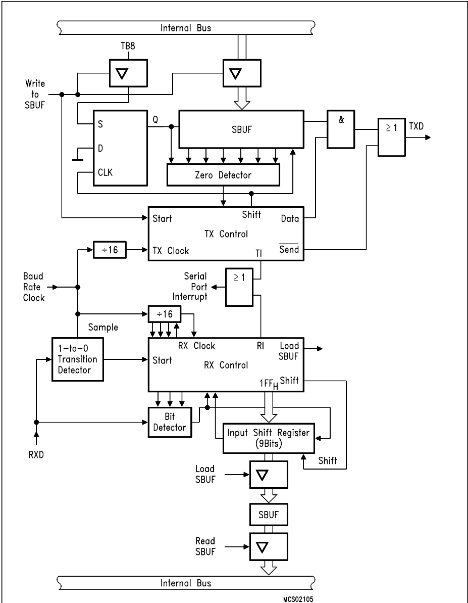
Figure 6-17a Serial Interface, Mode 2 and 3, Functional Diagram
