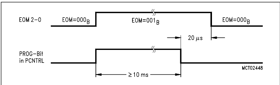
Figure 9-6 Erase Sequence
