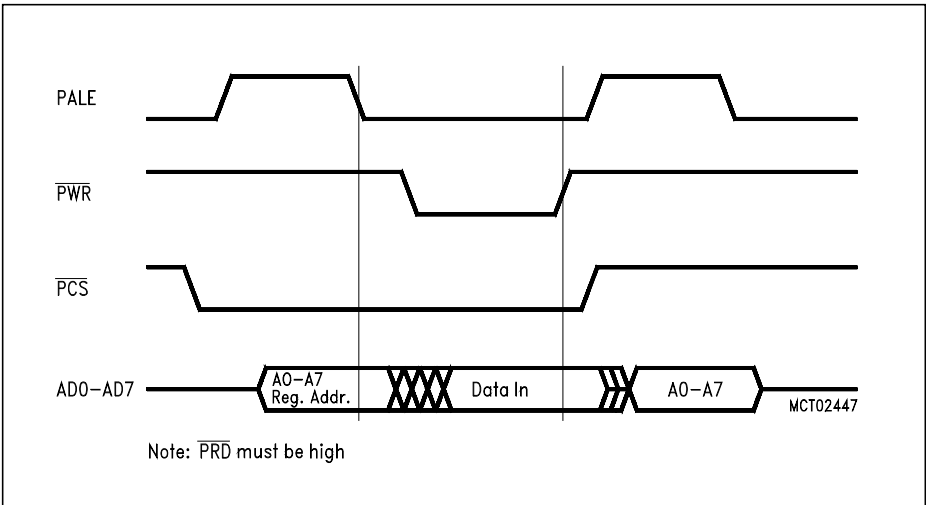
Figure 9-5 Program Interface Write Cycle
