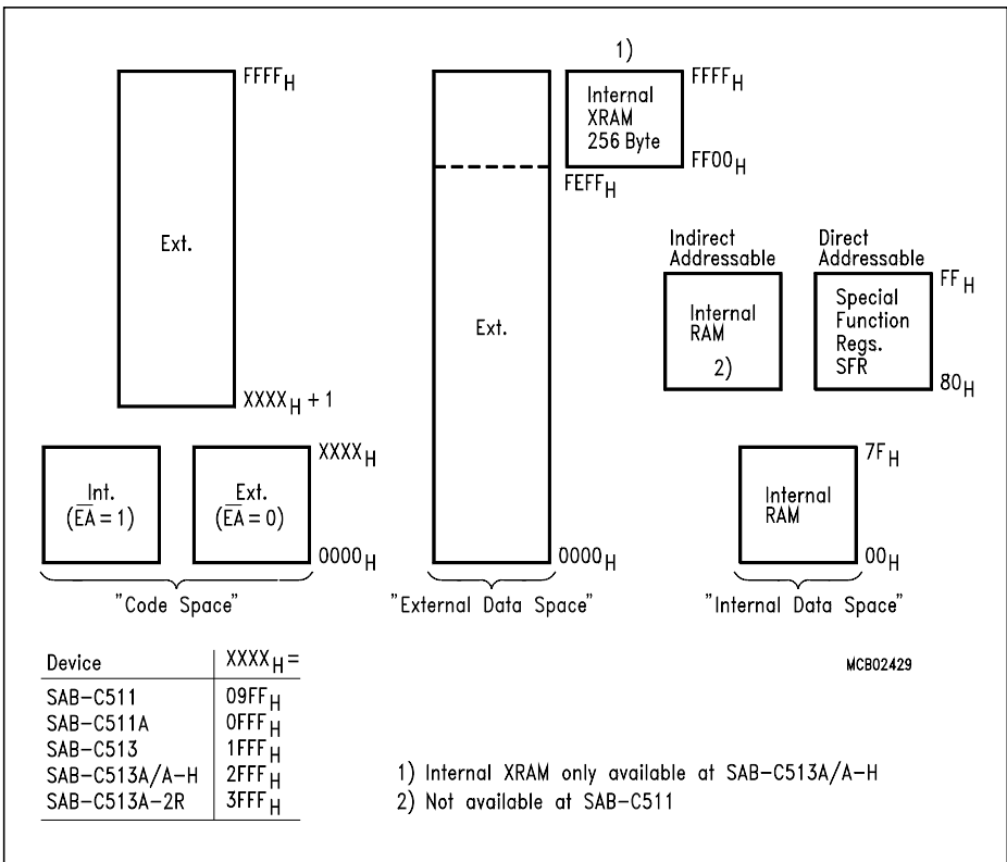
Figure 3-1 Memory Map
