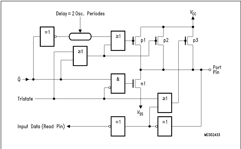
Figure 6-3c Driver Circuit of Port 1 pins P1.3 and P1.5 (when used for SRI and \overline{\text{SLS}} )
