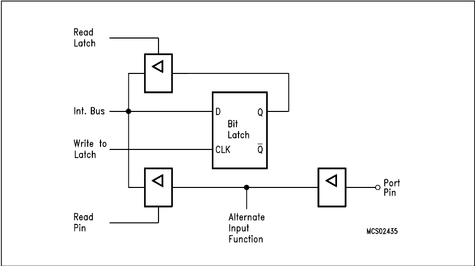
Figure 6-5b Port pins P1.2, P1.3 and P1.5 (when used as inputs to SSC)
