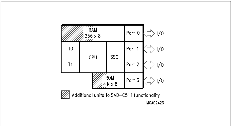
Figure 1-2 C511A Functional Units
