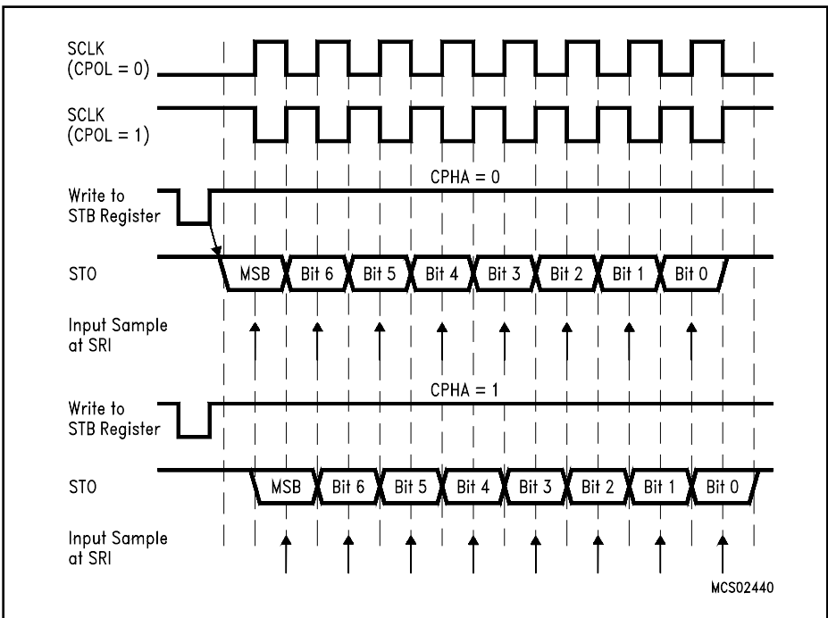
Figure 6-13 Master Mode Operation of SSC
