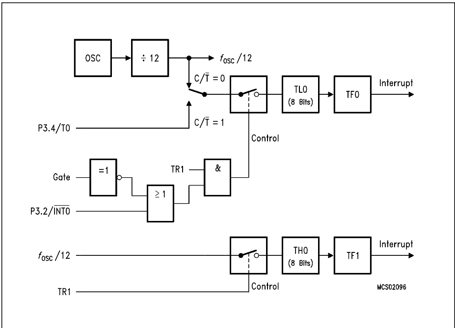
Figure 6-10 Timer/Counter 0, Mode 3: Two 8-Bit Timers/Counters
