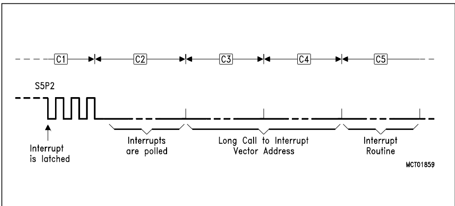
Figure 7-2 Interrupt Response Timing Diagram
