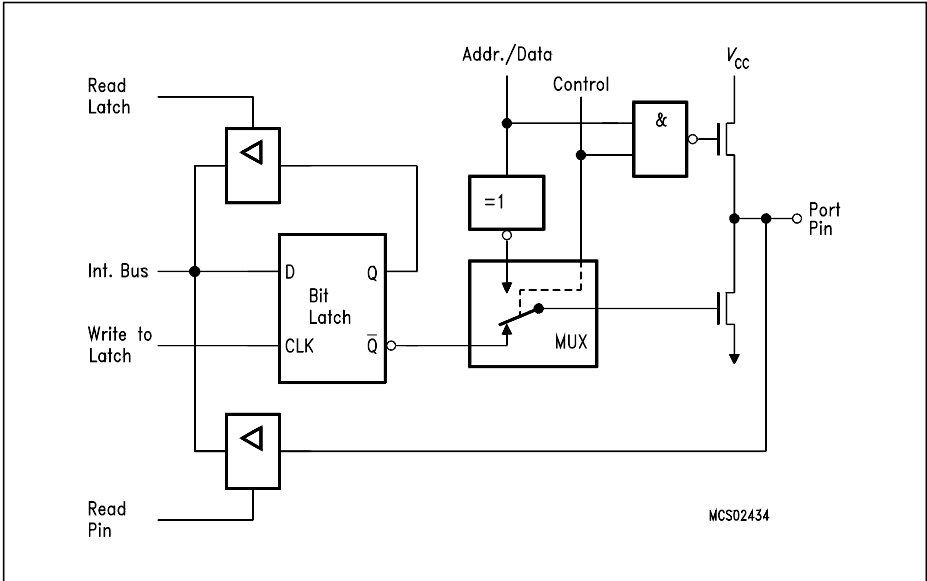
Figure 6-4a Port 0 Circuitry
