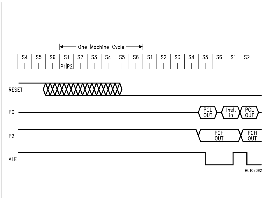
Figure 5-1 CPU Timing after Reset
