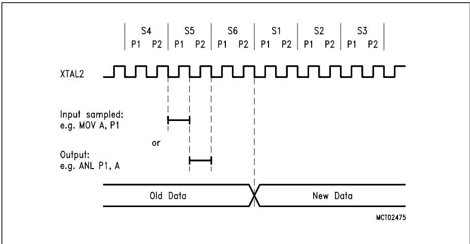
Figure 6-6 Port Timing
