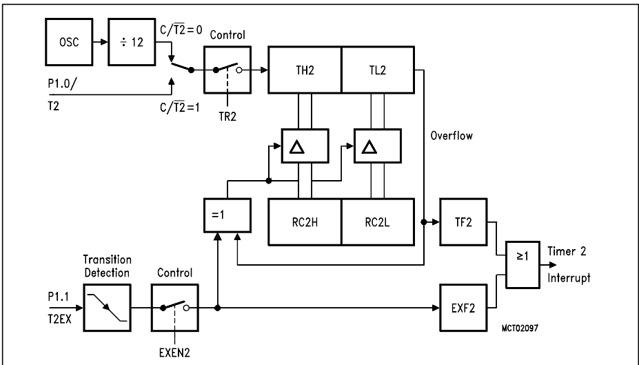
Figure 6-11 Timer 2 Auto-Reload Mode (DCEN = 0)
