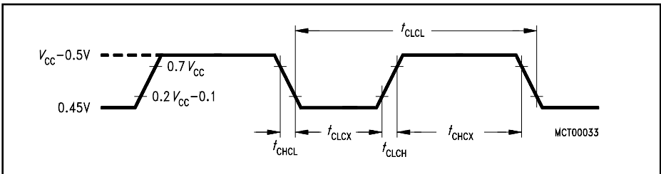
Figure 10-5 External Clock Drive at XTAL1
