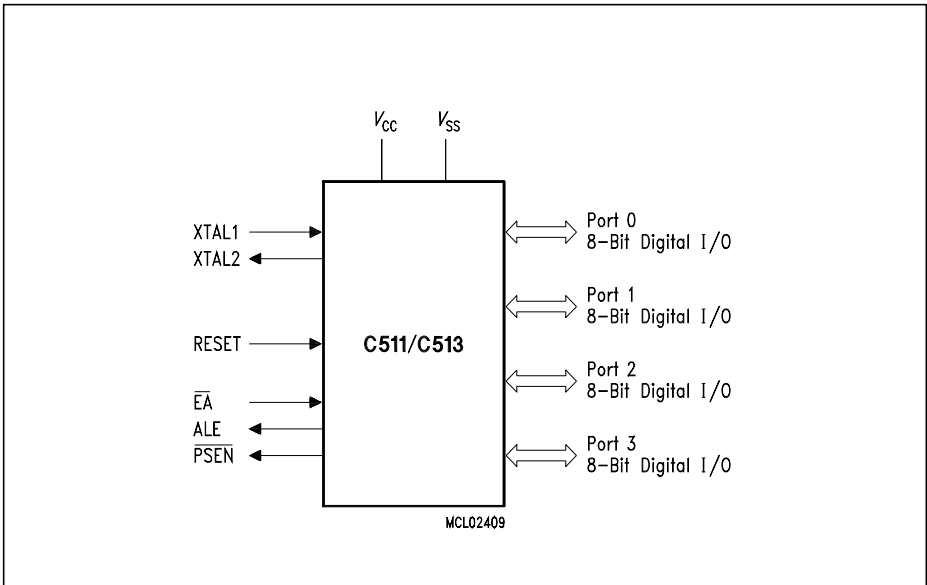
Figure 1-5 C511/C513 Logic Symbol
