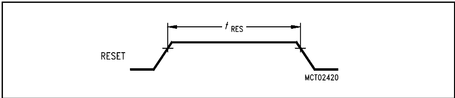
Figure 10-9 C513A-H Reset Pulse
