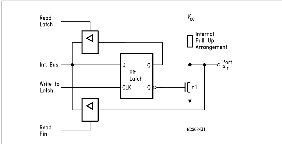
Figure 6-2 Basic Output Driver Circuit of Ports 1, 2 and 3
