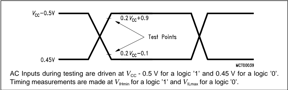
Figure 10-10 AC Testing: Input, Output Waveforms
