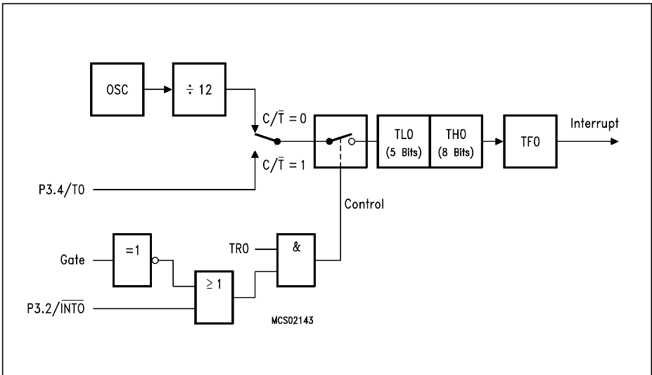
Figure 6-7 Timer/Counter 0, Mode 0: 13-Bit Timer/Counter
