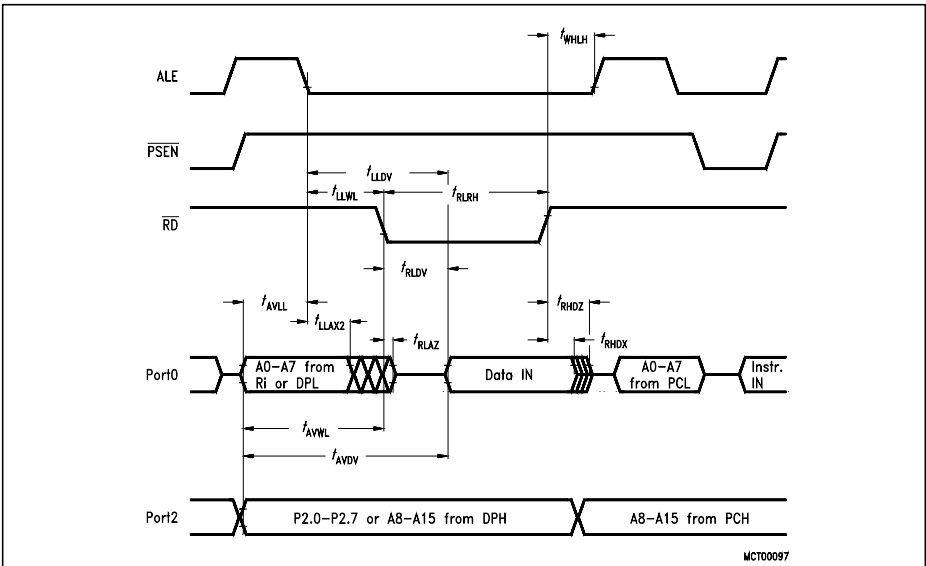
Figure 10-2 Data Memory Read Cycle
