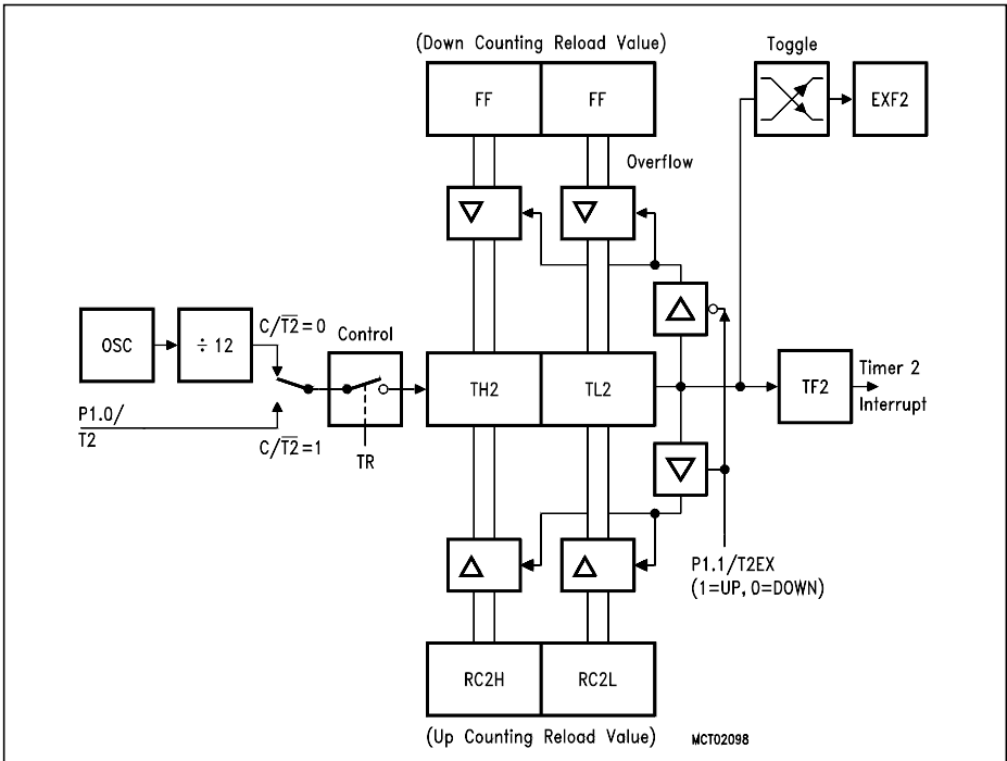
Figure 6-12 Timer 2 Auto-Reload Mode (DCEN = 1)
