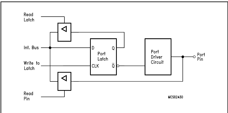
Figure 6-1 Basic Structure of a Port Circuitry
