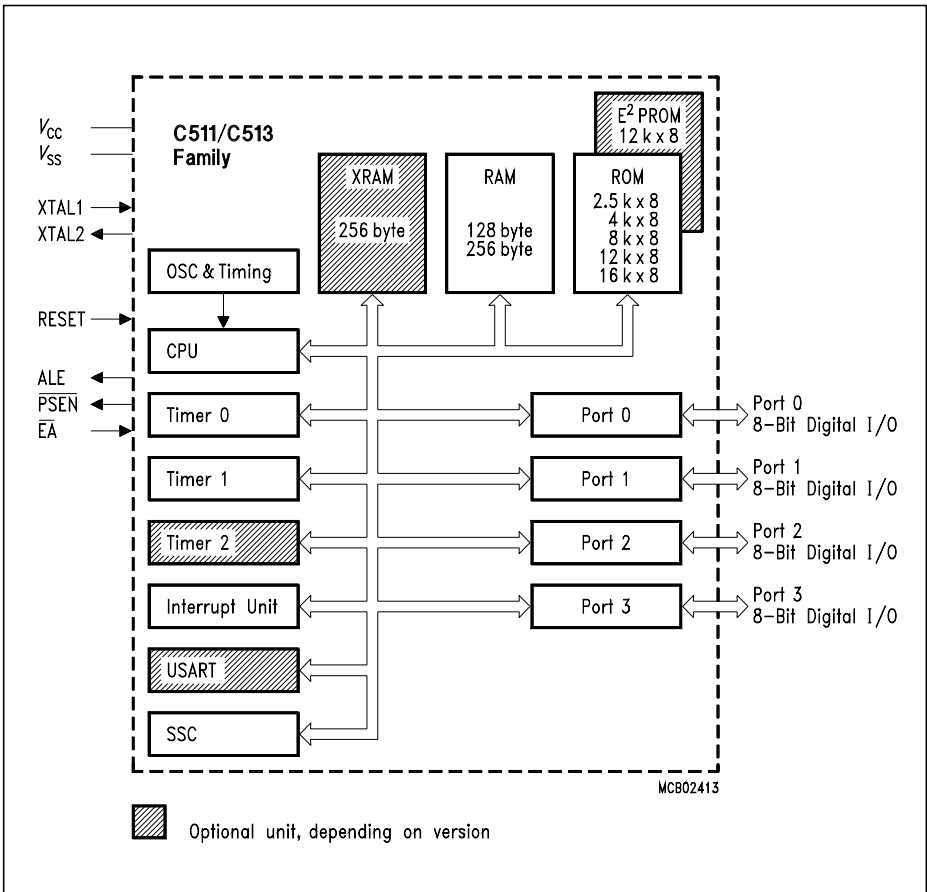
Figure 2-1 Block Diagram of the SAB-C511/513
