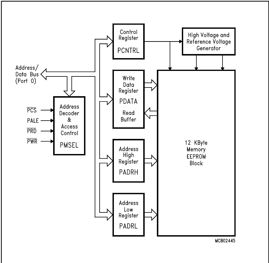
Figure 9-3 Block Diagram of the SAB-C513A-H Programming Interface
