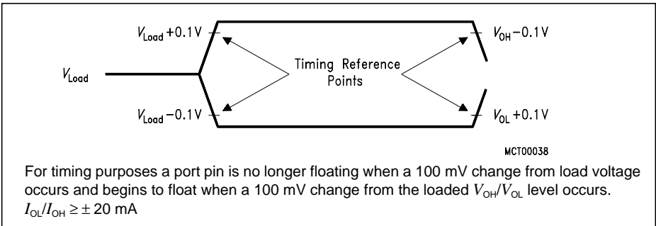
Figure 10-11 AC Testing: Float Waveforms
