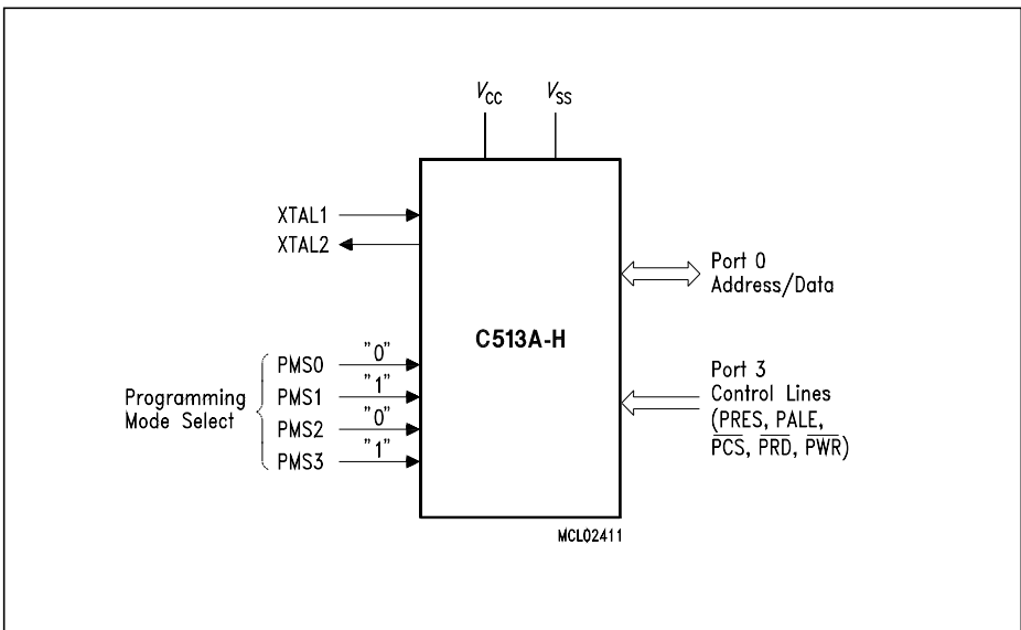
Figure 9-1 SAB-C513A-H Logic Symbol in Programming Mode
