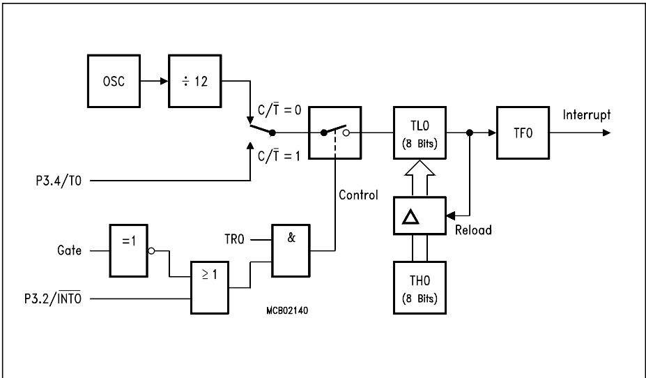
Figure 6-9 Timer/Counter 0, Mode 2: 8-Bit Timer/Counter with Auto-Reload
