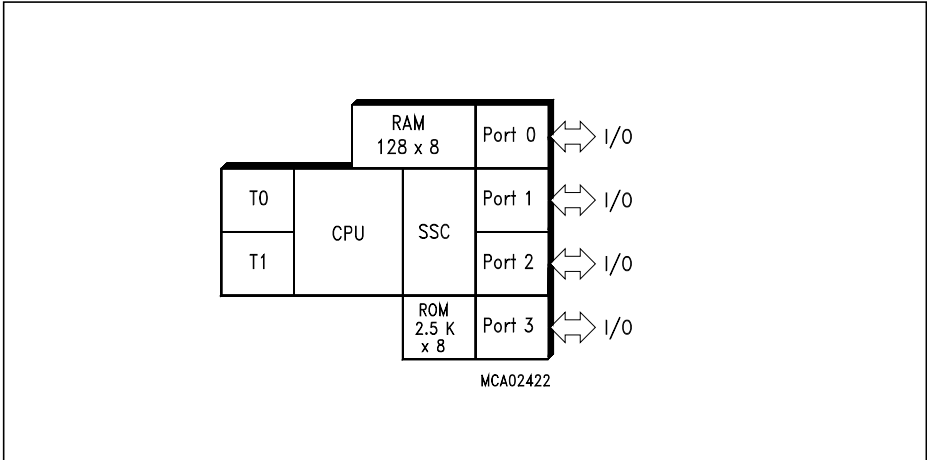
Figure 1-1 C511 Functional Units
