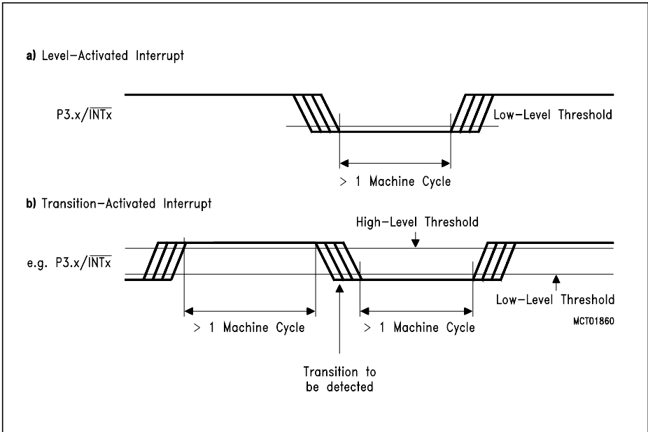
Figure 7-3 External Interrupt Detection
