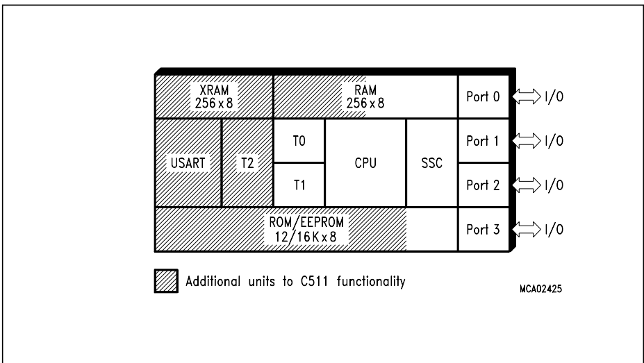
Figure 1-4 C513A / C513A-H Functional Units
