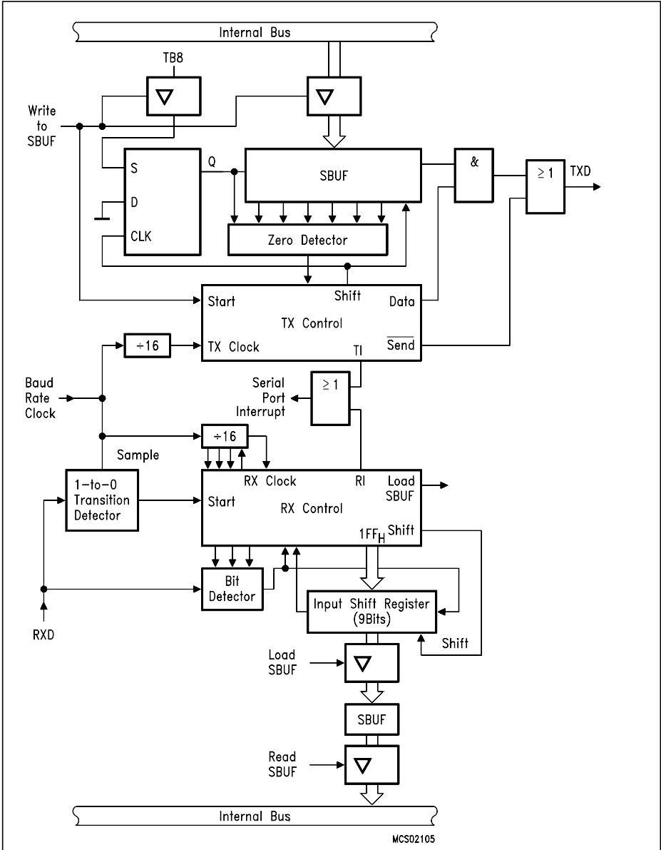
Figure 6-10a Serial Interface, Mode 2 and 3, Functional Diagram
