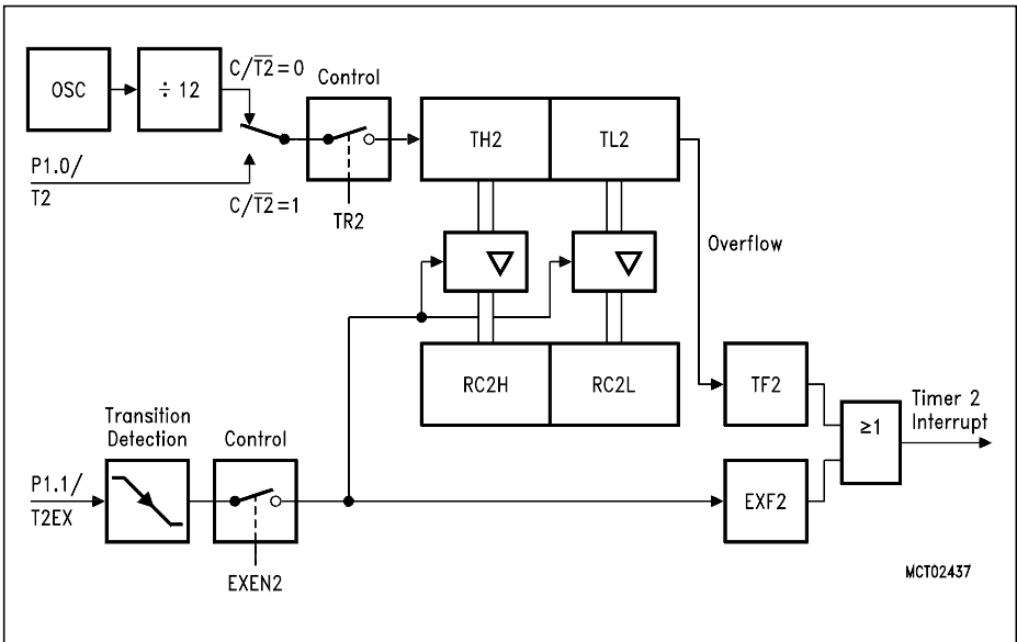
Figure 6-13 Timer 2 in Capture Mode
