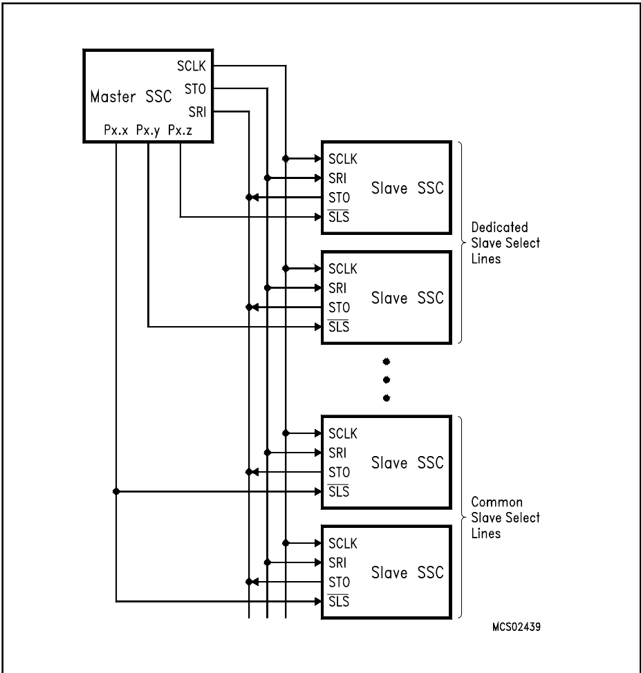
Figure 6-12 Typical SSC System Configuration
