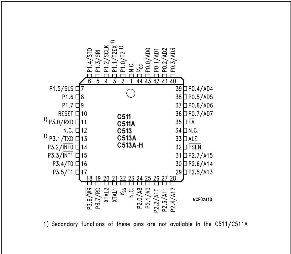
Figure 1-6 P-LCC-44 Package Pin Configuration (Top View)
