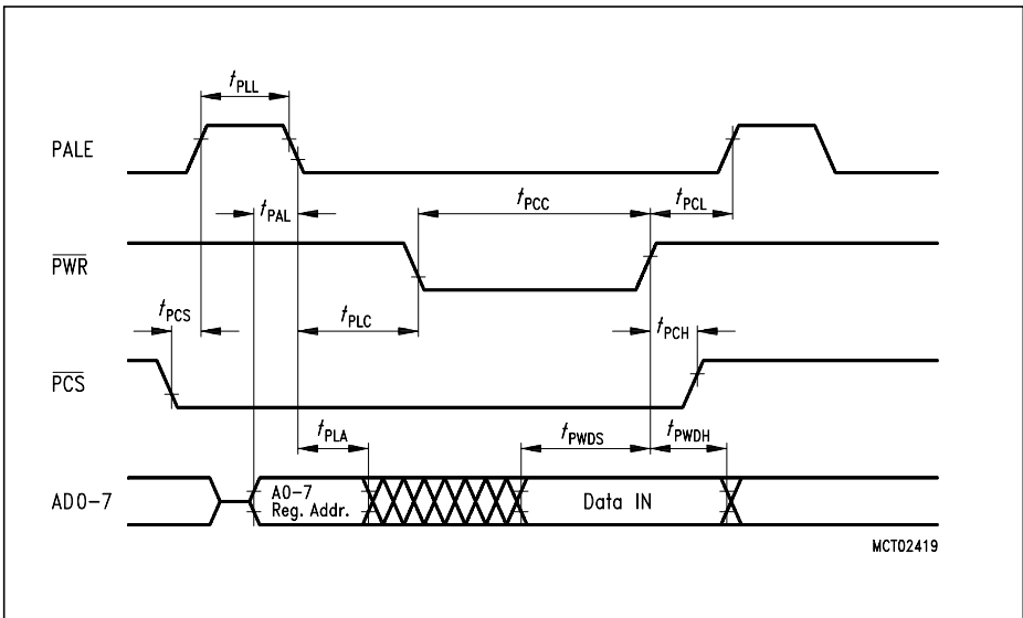
Figure 10-8 C513A-H Programming Interface Write Cycle
