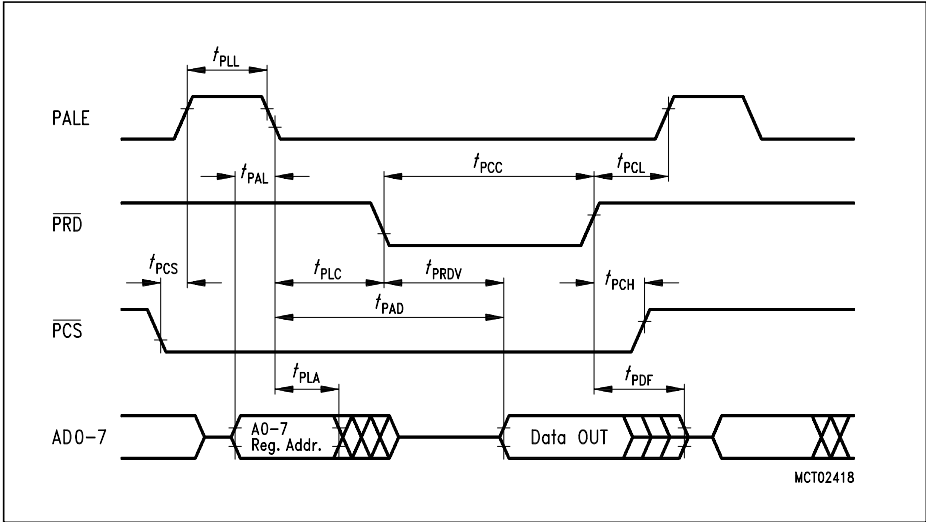
Figure 10-7 C513A-H Programming Interface Read Cycle
