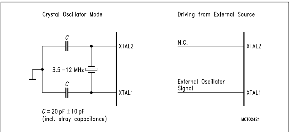
Figure 10-12 Recommended Oscillator Circuits for Crystal Oscillator
