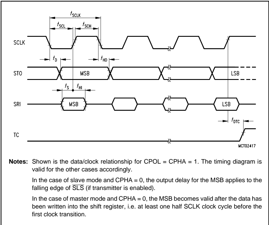
Figure 10-4 SSC Timing
