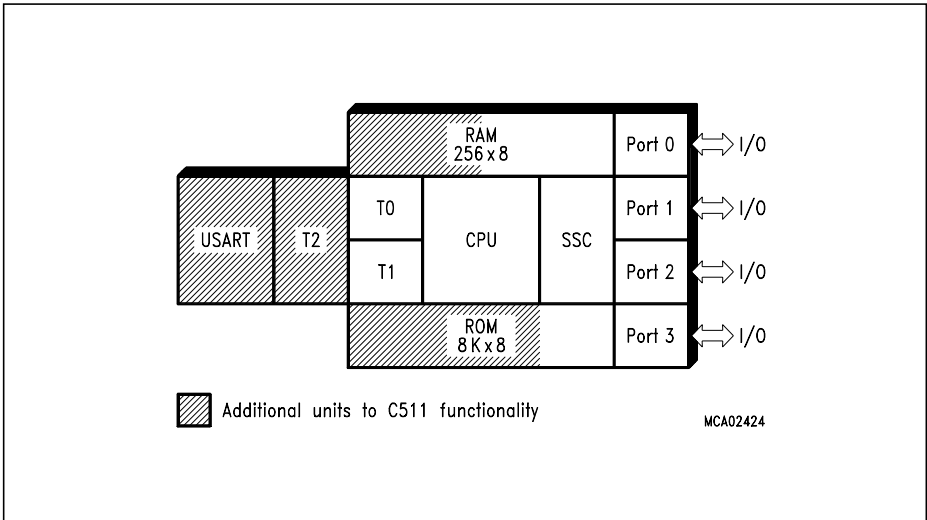
Figure 1-3 C513 Functional Units
