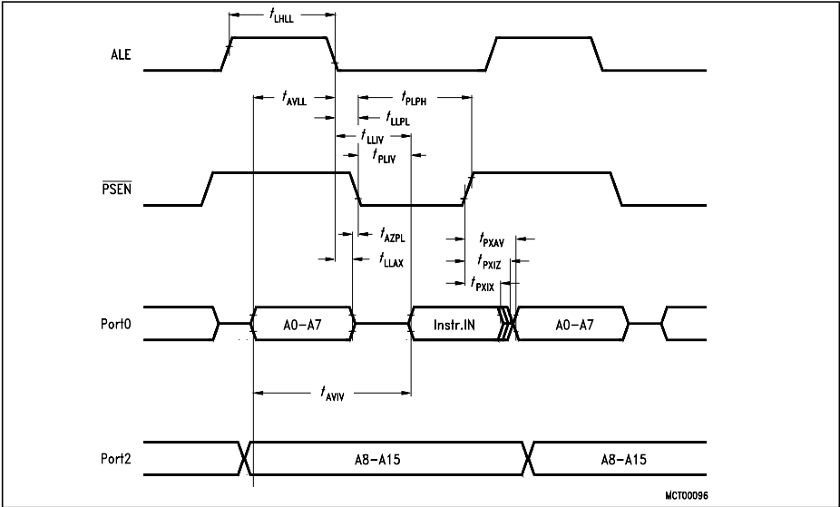
Figure 10-1 Program Memory Read Cycle
