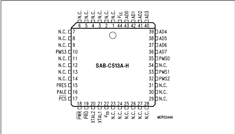
Figure 9-2 SAB-C513A-H Pin Configuration in Programming Mode
