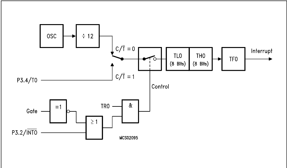
Figure 6-8 Timer/Counter 0, Mode 1: 16-Bit Timer/Counter
