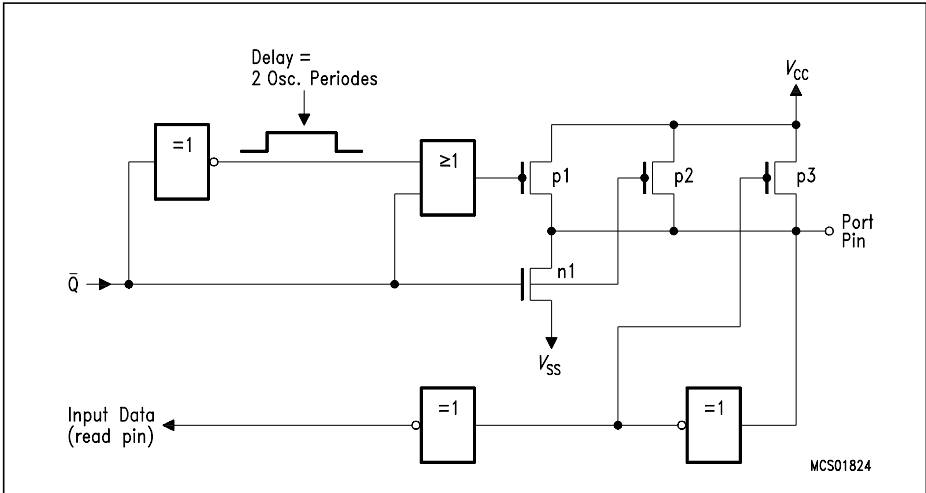
Figure 6-3a Output Driver Circuit of Ports 1, 2 and 3 (except P1.2, P1.3, P1.4 and P1.5)
