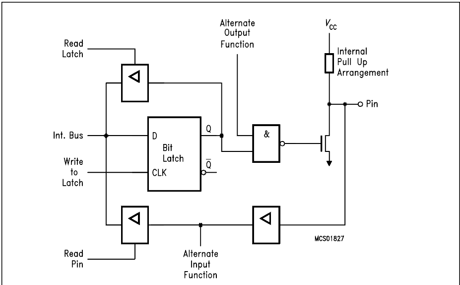
Figure 6-5a Ports 1 and 3
