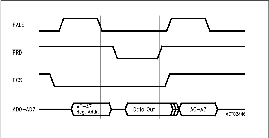
Figure 9-4 Program Interface Read Cycle
