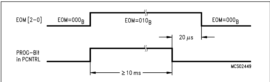
Figure 9-7 Write (Programming) Sequence
