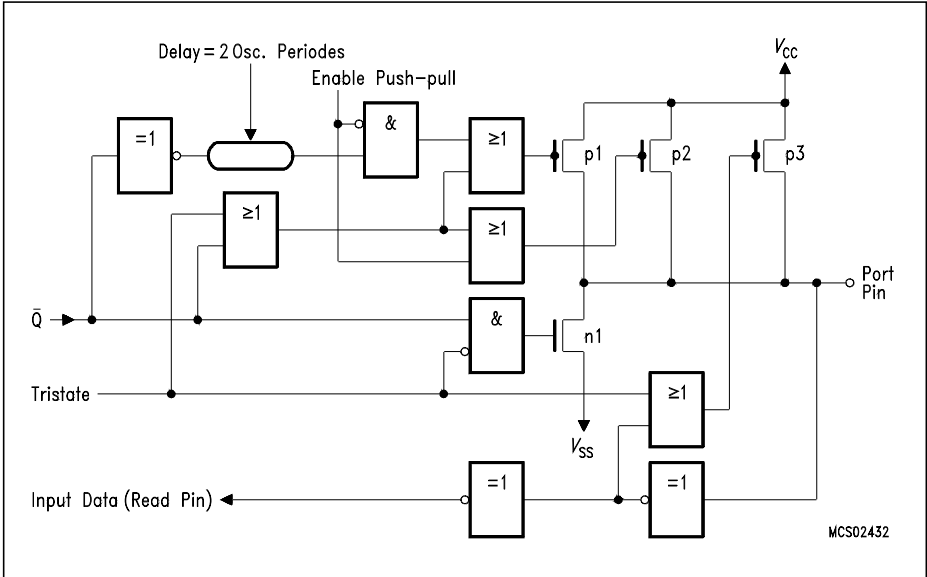
Figure 6-3b Driver Circuit of Port 1 pins P1.2 and P1.4 (when used for SCLK and STO)
