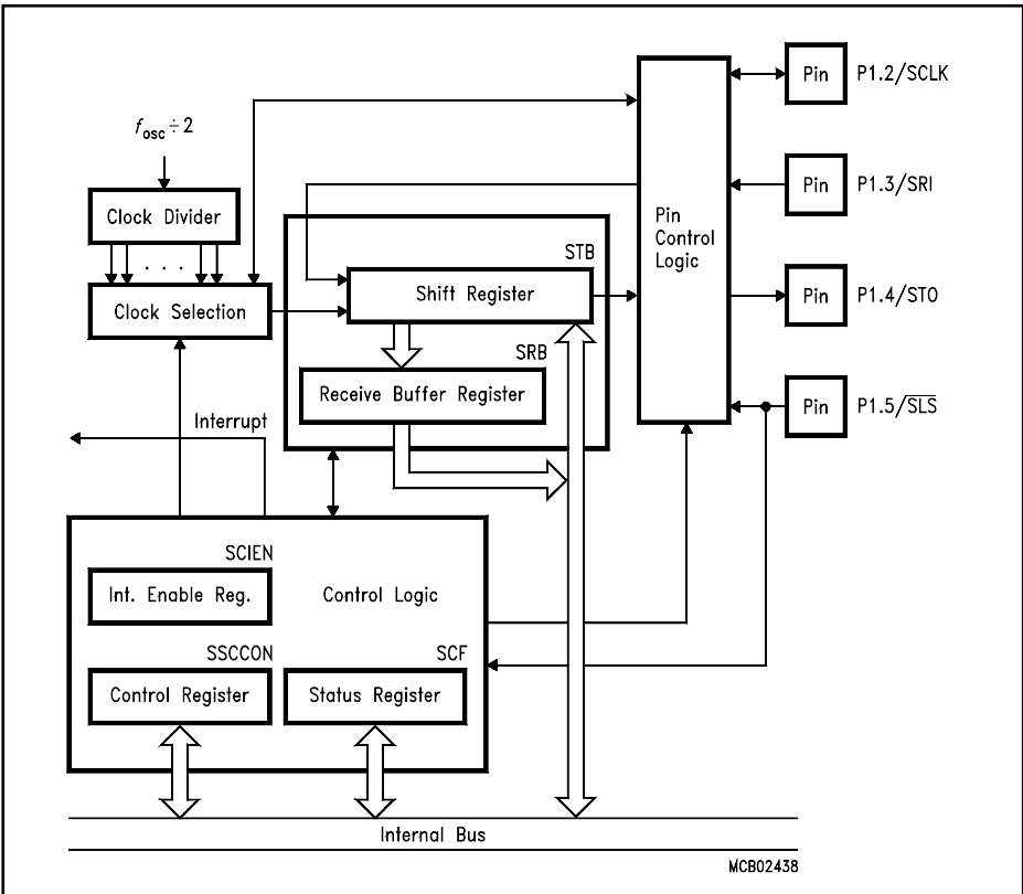
Figure 6-11 SSC Blockdiagram
