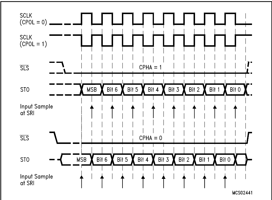
Figure 6-14 Slave Mode Operation of SSC
