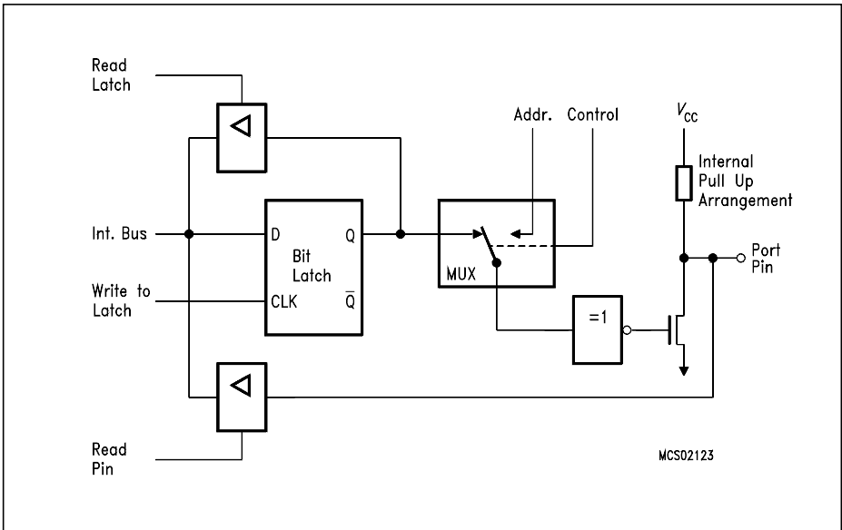
Figure 6-4b Port 2 Circuitry
