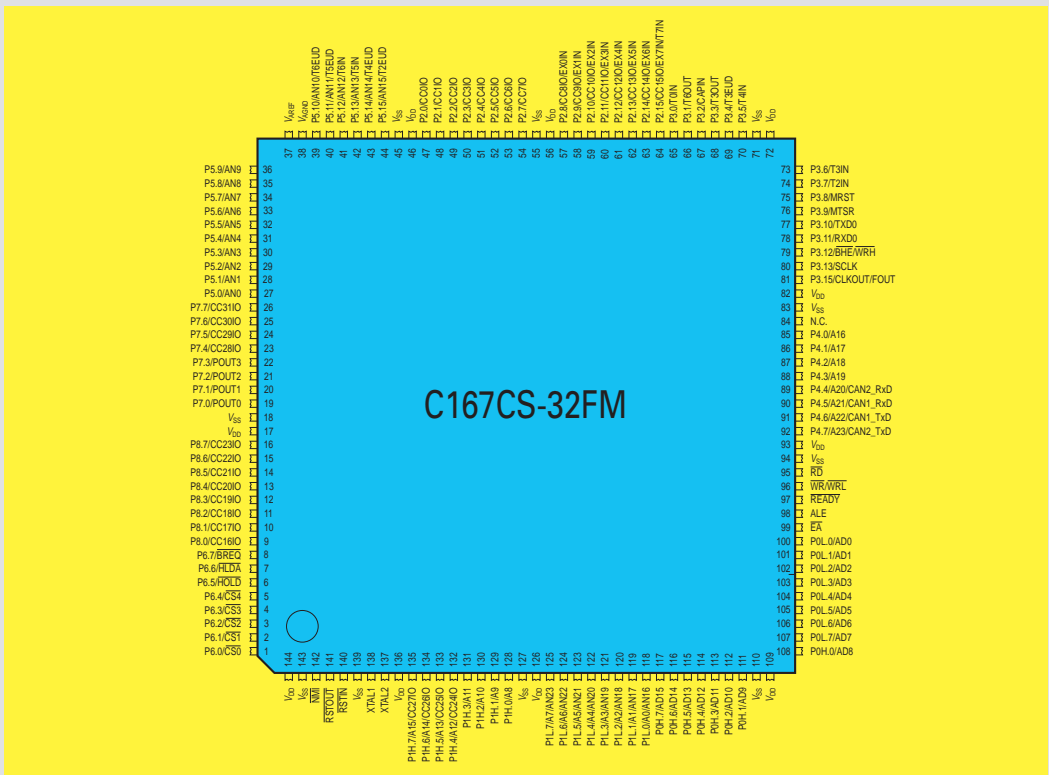
C167CS-32FM: PIN CONFIGURATION
