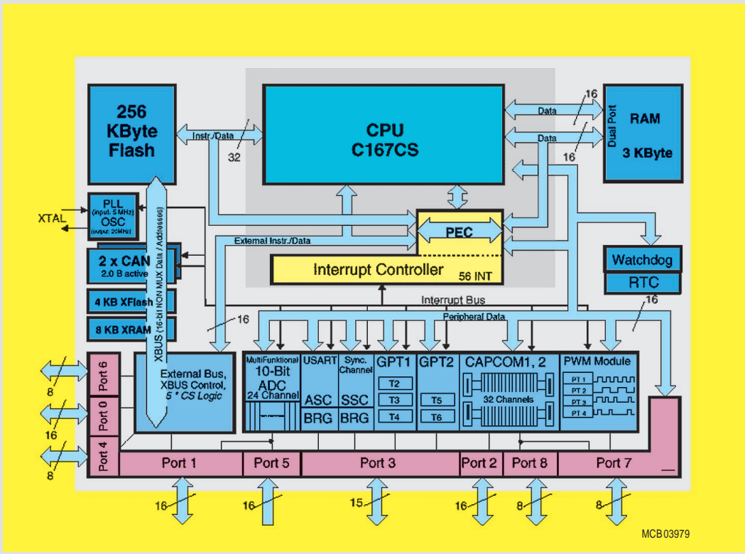
C167CS-32FM: BLOCK DIAGRAM
